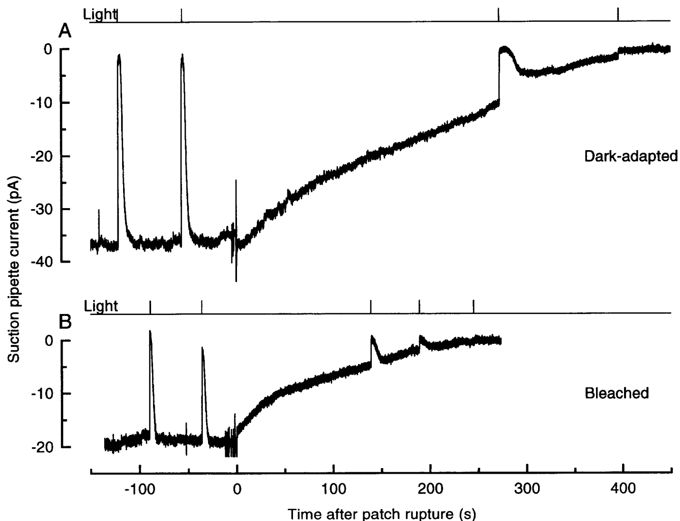
FIGURE 2. Suction pipette current recorded during the introduction of GTP- \gamma -S in complete darkness ( A ) into a dark-adapted rod or ( B ) into a rod exposed 70 min earlier to intense illumination which bleached 26% of the photopigment. The outer segment was drawn into the suction pipette, a patch pipette containing a solution which included 2 mM GTP- \gamma -S sealed onto the protruding inner segment, and the patch ruptured at time zero to establish the whole-cell recording configuration. Flash monitor indicates infrequent just-saturating flashes which delivered A , 150 and B , 310 photons \mu\text{m}^{-2} .
