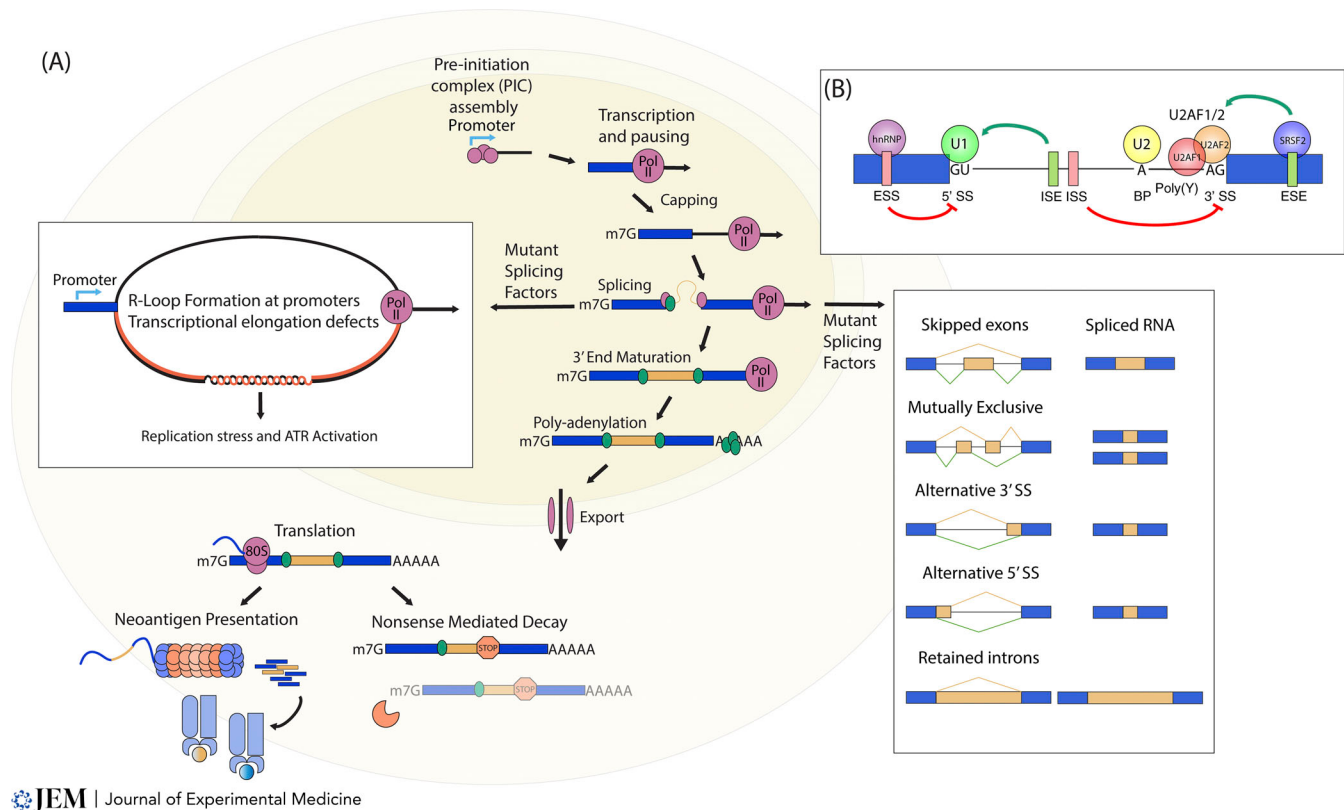
Figure 1. Normal RNA splicing, 5'-end capping, and 3'-end cleavage and polyadenylation. (A) Transcription and RNA processing begin with assembly of the pre-initiation complex on gene promoters, followed by recruitment of RNA polymerase II, and 5' pausing. RNA transcription (blue bar), 5' capping, and splicing occur cotranscriptionally on nascent RNA. These processes are facilitated by the recruitment of protein cofactors that facilitate capping, exon junction complex formation, and splicing (green dots). 3'-end maturation and polyadenylation then occur and release the RNA, allowing it to be exported into the cytoplasm. Splicing dysregulation, cellular stress, and the presence of mutant splicing factors can lead to the formation of tripartite DNA/RNA structures (R-loops) and downstream genomic instability. Different patterns of RNA splicing can occur (left: gold and green lines) and consequently lead to changes in the downstream RNA (right column). These changes can include the inclusion of novel sequences (gold bars) within the transcript of interest (blue bars). Once the mature alternatively spliced RNA is exported from the nucleus, it undergoes translation in the cytoplasm. Consequences of translation can lead to (left) translation of protein and eventual possible presentation on cell surface MHC molecules (blue and gold circles). Alternatively, the presence of a premature stop codon (red stop sign) can cause recruitment of the RNA degradation machinery (orange pac-man) and RNA downregulation through nonsense-mediated decay. (B) Binding of splicing factors to the RNA and regulation through cis and trans elements. Enhancers (green box, green arrow) and silencers (red box, red arrow) of splicing can be present in the intron (ISE, ISS) or exon (ESE, ESS). These sequences can be recognized by RNA binding proteins such as hnRNP (purple circle) or SRSF2 (blue circle) and promote (green arrow) or repress (red arrow) alternative splicing patterns.
