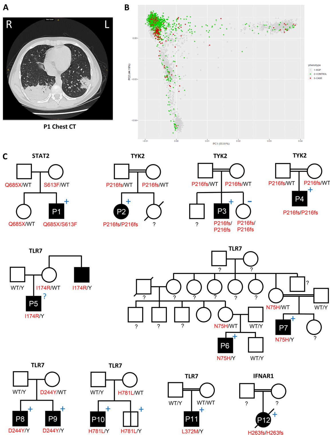
Figure 1. Recessive inborn errors of the type I IFN pathway underlie life-threatening viral infections. (A) Chest computed tomography scan on day 6 after disease onset in P1, showing ground-glass opacification and consolidation in both lungs. (B) PCA analysis of patients and controls. KGP, 1000 Genomes Project database. (C) Pedigrees and familial segregation of the variants identified. Black symbols, patients with moderate to critical COVID-19 pneumonia; symbols with vertical bars, individuals with asymptomatic SARS-CoV-2 infection; blue + and - symbols, seropositive and seronegative for SARS-CoV-2, respectively.
