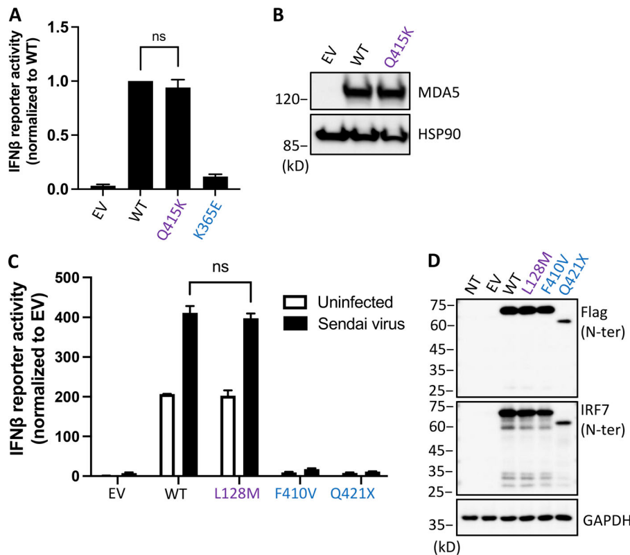
Figure 3. Functional tests of biallelic variants identified in the control cohort.
