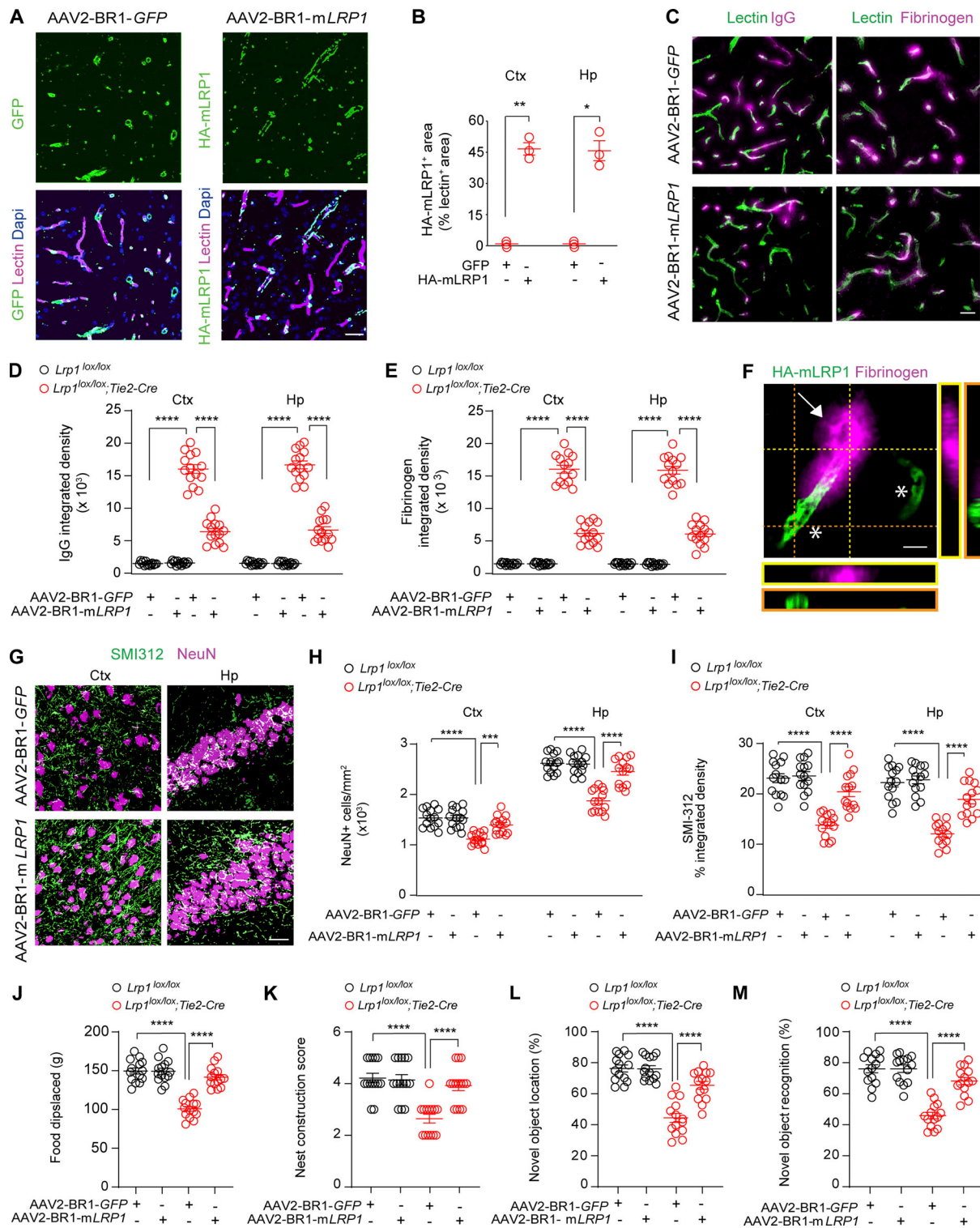
Figure 3. Rescue of vascular and neuronal phenotype in Lrp1^{lox/lox}; Tie2-Cre mice by endothelial-specific LRP1 gene replacement. (A and B) Endothelial expression of GFP (left, green), HA-tagged mLRP1 (right, green), and lectin + endothelium (purple) in the cortex of 4-mo-old Lrp1^{lox/lox}; Tie2-Cre mice after AAV2-BR1-GFP (left) or AAV2-BR1-mLRP1 (LRP1 minigene, right) treatment (A), and quantification of HA-mLRP1 + area colocalized with lectin + endothelial capillary profiles (<6 \mu m in diameter) in the cortex (Ctx) and hippocampus (Hp; B). Scale bar = 25 \mu m. Mean \pm SEM; n = 3 mice/group. (C–E) IgG (left, purple) and fibrinogen (right, purple) perivascular capillary deposits (C) and quantification (D and E) in 4-mo-old Lrp1^{lox/lox}; Tie2-Cre and Lrp1^{lox/lox} mice after AAV2-BR1-GFP (top) or AAV2-BR1-mLRP1 (bottom) treatment. Green, lectin + endothelium. Scale bar = 20 \mu m. Mean \pm SEM, n = 14 mice/group. (F) High-magnification confocal images from Lrp1^{lox/lox}; Tie2-Cre mouse treated with AAV2-BR1-mLRP1 showing that vessel segments that reexpress HA-mLRP1 (asterisks) were no longer leaky compared with a vessel segment that does not express HA-mLRP1 (arrow) that leaks fibrinogen. Scale bar = 10 \mu m. (G–I) NeuN + neurons and SMI312 + neurites (G) and quantification of NeuN + neurons and SMI312 + neurites in the cortex and hippocampus of 4-mo-old Lrp1^{lox/lox} and Lrp1^{lox/lox}; Tie2-Cre mice after AAV2-BR1-GFP (top panels) or AAV2-BR1-mLRP1 (bottom panels) treatment (H and I). Scale bar = 50 \mu m. Mean \pm SEM, n = 14 mice/group. (J–M) Burrowing (J), nest
