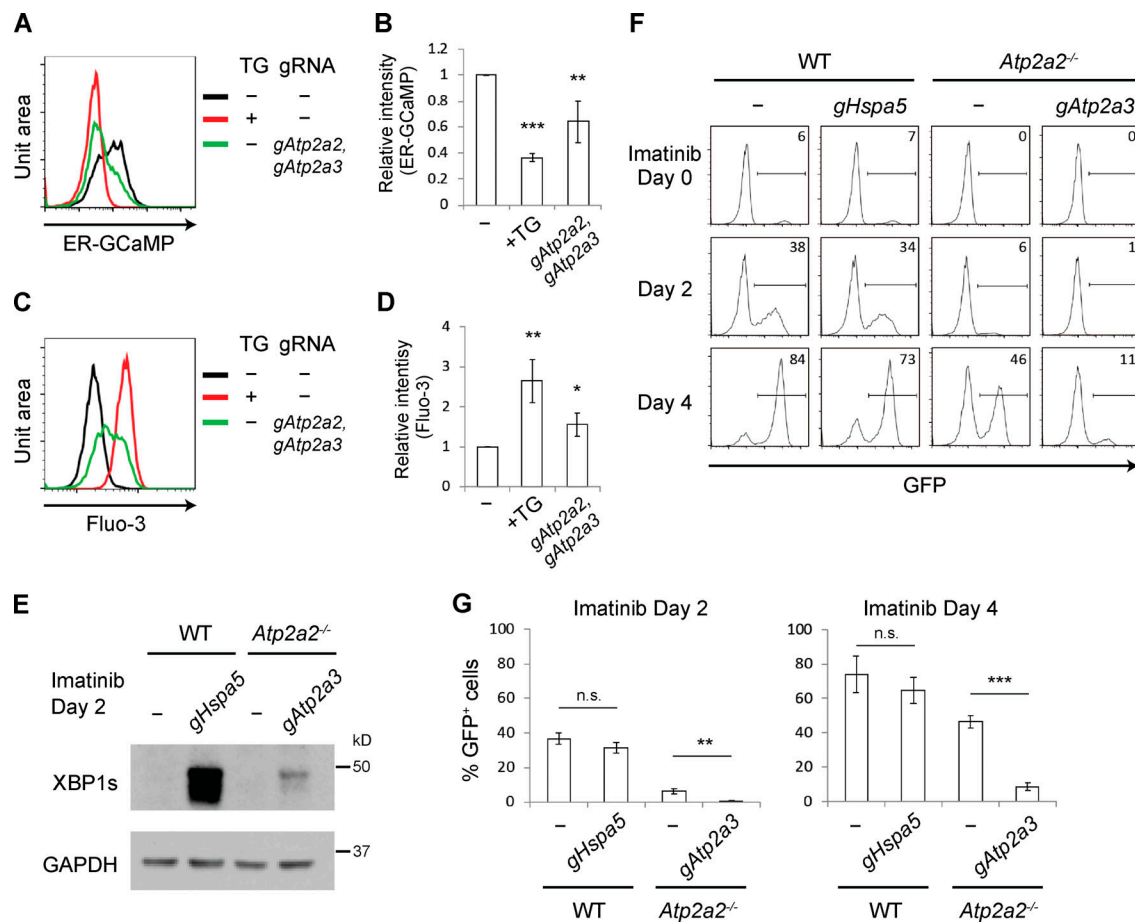
Figure 3. Loss of SERCA2 and SERCA3 disrupts \text{Ca}^{2+} homeostasis. (A–D) Flow-cytometric analysis of WT abl preB cells expressing ER-GCaMP6-150 (A) or incubated with Fluo-3 AM \text{Ca}^{2+} indicator (C) without further treatment (black histogram), treated with thapsigargin (TG; red histogram), or after bulk inactivation of Atp2a2 and Atp2a3 genes (green histogram). Median fluorescence intensity was calculated and normalized to that of the black histogram in each experiment to derive the relative intensity of ER-GCaMP6-150 (B; mean \pm SD; n = 4 ) and Fluo-3 dye (D; mean \pm SD; n = 3 ). *, P < 0.05 ; **, P < 0.01 ; ***, P < 0.001 compared with the untreated sample. (E) Western blot analysis of XBP1s in imatinib-treated WT abl preB cells bulk Hspa5 ( gHspa5 ) inactivated or Atp2a2 -/- cells bulk Atp2a3 ( gAtp2a3 ) inactivated ( n = 3 ). (F) Flow-cytometric analysis of GFP expression from pMGINV rearrangement in cells from E treated with imatinib for 0, 2, or 4 d. (G) Mean \pm SD of three pMGINV experiments performed as in F. **, P < 0.01 ; ***, P < 0.001 . n.s., not significant.
