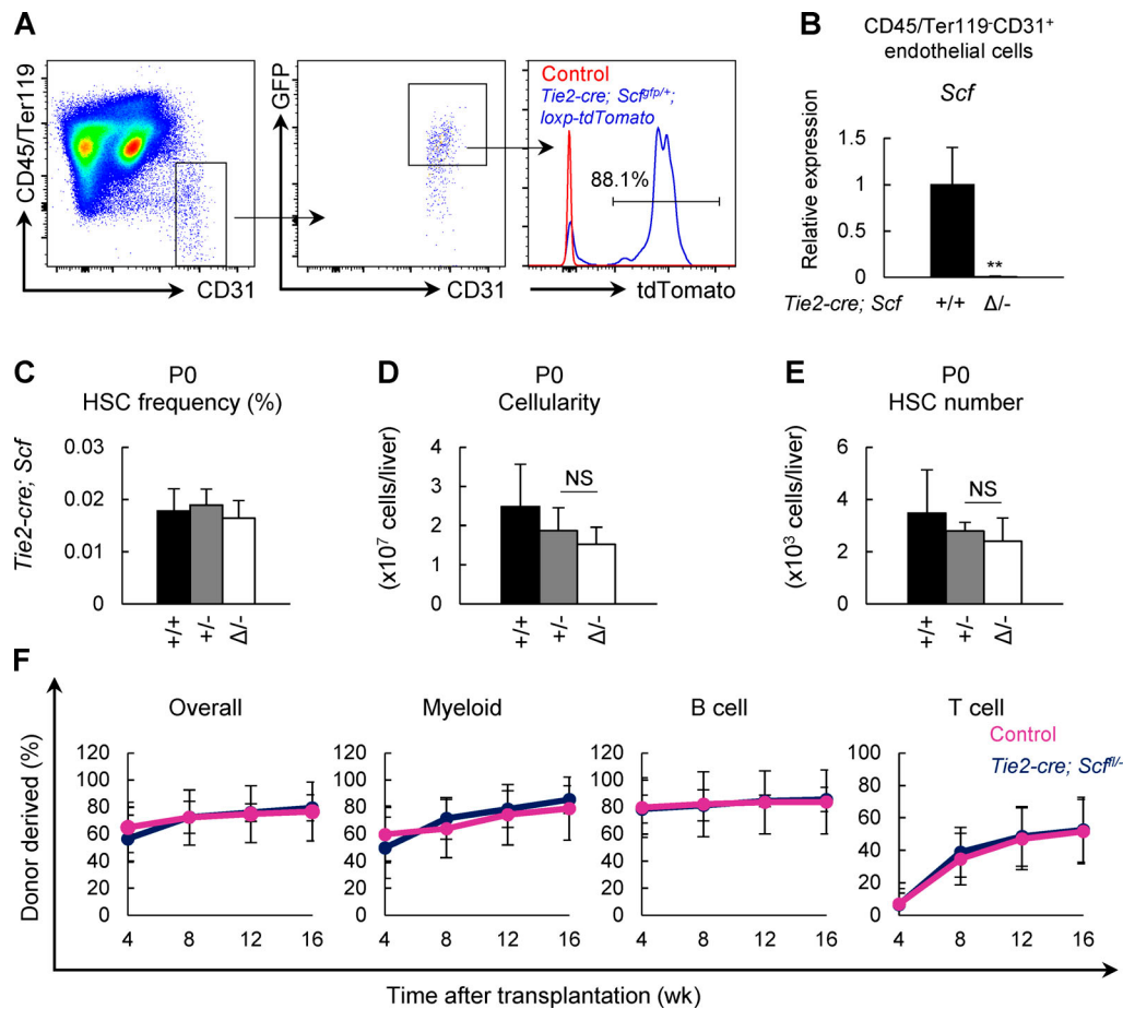
Figure 6. Deletion of Scf from endothelial cells does not lead to significant reduction in HSC frequency or function in the developing liver. (A) Tie2-cre recombined in the majority of CD45-Ter119-CD31 + - Scf -GFP + endothelial cells in the Tie2-cre ; Scf flp/+ ; loxp-tdTomato P0 livers ( n = 5 mice for control, and n = 3 mice for Tie2-cre ; Scf flp/+ ; loxp-tdTomato ). (B) qRT-PCR analysis of Scf transcript levels in CD45-Ter119-CD31 + endothelial cells sorted from P0 livers of control or Tie2-cre ; Scf flp/+ mice ( n = 3 mice for control, and n = 4 mice for Tie2-cre ; Scf flp/+ ). (C-E) HSC frequency (C), liver cellularity (D), and HSC number (E) in P0 Tie2-cre ; Scf flp/+ mice compared with littermate controls ( n = 7 mice for Scf +/+ , n = 3 mice for Scf flp/+ , and n = 9 mice for Tie2-cre ; Scf flp/+ ). (F) 5 \times 10^5 liver cells from Tie2-cre ; Scf flp/+ mice gave normal levels of reconstitution in irradiated mice (data represent three independent experiments with a total of n = 15 recipients for controls and n = 16 recipients for mutants). Scf +/+ and Scf flp/+ mice were used as controls. +, WT allele; Δ, recombined Scf flp allele; -, germline deleted allele. Scf +/+ mice include Cre ; Scf +/+ , Cre ; Scf flp/+ , and Cre (-); Scf +/+ mice. Scf flp/+ mice include Cre ; Scf flp/+ and Cre (-); Scf flp/+ mice. All data represent mean \pm SD. Two-tailed Student's t tests were used to evaluate statistical significance. **, P < 0.01 .
