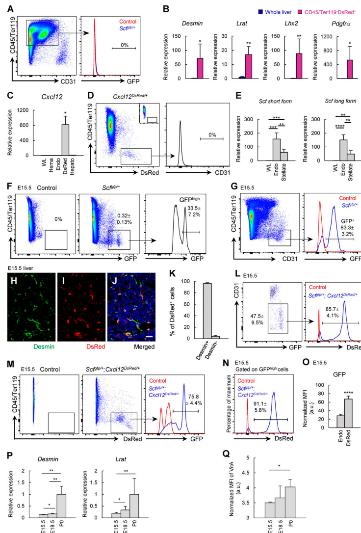
Figure S2. Endothelial cells and hepatic stellate cells are the major sources of SCF in the developing liver. (A) Representative flow-cytometric plots showing that CD45 + Ter119 + hematopoietic cells from livers of P0 Scf flp/+ mice did not express Scf -GFP ( n = 5 mice for control, and n = 5 mice for Scf flp/+ ). (B) CD45 + Ter119 + Cxcl12 -DsRed + stromal cells had significantly higher expression of Desmin , Lrat , Lhx2 , and Pdgfra compared with whole P0 liver cells as revealed by qRT-PCR analysis ( n = 5 for whole P0 liver cells, and n = 3 for CD45 + Ter119 + Cxcl12 -DsRed + cells). (C) Cxcl12 transcript levels in different cell populations of P0 liver as quantified by qRT-PCR ( n = 3 for whole liver cells [WL], n = 3 for CD45 + or Ter119 + hematopoietic cells [Hema], n = 3 for CD45 + Ter119 + CD31 + endothelial cells [Endo], n = 4 for CD45 + Ter119 + Cxcl12 -DsRed + stellate cells [DsRed], and n = 4 for CD45 + Ter119 + tdTomato + hepatocyte lineage cells from Albumin-cre; loxP-tdTomato mice [Hepato]). Cxcl12 was highly expressed by Cxcl12 -DsRed + hepatic stellate cells with little if any expressed by other cells in the P0 liver. (D) Representative flow-cytometric plots of enzymatically digested P0 Cxcl12 DsRed/+ livers show that CD45 + Ter119 + Cxcl12 -DsRed + stromal cells did not express CD31, an endothelial cell marker ( n = 5 mice from two independent experiments). (E) qRT-PCR analysis of short and long forms of Scf transcript levels in endothelial and stellate cells of P0 livers ( n = 5 for WL, n = 3 for Endo, and n = 5 for DsRed + stellate cells). (F) Representative flow-cytometric plots showing that Scf -GFP was expressed by rare nonhematopoietic cells in E15.5 livers. Among Scf -GFP + stromal cells, there was a subset that expressed higher levels of Scf -GFP, denoted as GFP high ( n = 3 embryos for control, and n = 6 embryos for Scf flp/+ ). (G) Representative flow-cytometric plots showing that the majority of CD45 + Ter119 + CD31 + endothelial cells in the E15.5 livers expressed Scf -GFP ( n = 3 embryos for control, and n = 6 embryos for Scf flp/+ ). (H-I) Representative confocal images showing that virtually all Cxcl12 -DsRed + cells expressed Desmin , a stellate cell marker, in the E15.5 liver. (J) Quantification of Cxcl12 -DsRed + cells that expressed Desmin in E15.5 Cxcl12 DsRed/+ livers. The data are from three independent confocal images. (K) Representative flow-cytometric plots showing that the majority of CD45 + Ter119 + CD31 + Scf -GFP + nonendothelial stromal cells were Cxcl12 -DsRed + stellate cells in E15.5 livers ( n = 3 embryos for control, and n = 3 embryos for Scf flp/+ ; Cxcl12 DsRed/+ ). Note that at this stage, stellate cells expressed higher levels of Scf compared with endothelial cells. (L) The majority of CD45 + Ter119 + Cxcl12 -DsRed + stellate cells express Scf -GFP in Scf flp/+ ; Cxcl12 DsRed/+ mice ( n = 3 embryos for control, and n = 3 embryos for Scf flp/+ ; Cxcl12 DsRed/+ ). (M) The vast majority of CD45 + Ter119 + GFP high cells, denoted as GFP high cells in F, were Cxcl12 -DsRed + stellate cells in E15.5 livers ( n = 3 embryos for control, and n = 3 embryos for Scf flp/+ ; Cxcl12 DsRed/+ ). (N) CD45 + Ter119 + Cxcl12 -DsRed + cells expressed higher levels of Scf -GFP compared with CD45 + Ter119 + CD31 + endothelial cells in the Scf flp/+ E15.5 livers. The fluorescence intensity of GFP in CD45 + Ter119 + hematopoietic cells in each sample was used for normalization of the expression of Scf -GFP + ( n = 6 for Endo, and n = 3 for DsRed + stellate cells). (O) qRT-PCR analyses show that CD45 + Ter119 + Cxcl12 -DsRed + cells gradually up-regulated the expression of Desmin and Lrat during development ( n = 4-7 embryos or mice per time point). (P) CD45 + Ter119 + Cxcl12 -DsRed + stellate cells gradually up-regulate the accumulation of vitamin A (VitA; n = 3-6 embryos or mice per time point). All data represent mean \pm SD. Two-tailed Student's t tests were used to evaluate statistical significance. *, P < 0.05 ; **, P < 0.01 ; ***, P < 0.001 ; ****, P < 0.0001 . Scale bar is 20 \mu m in J. a.u., arbitrary units; MFI, mean fluorescence intensity.
