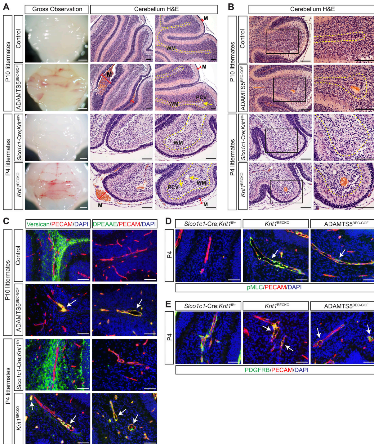
Figure 4. Forced expression of ADAMTS5 in BECs confers a vascular phenotype closely resembling early CCMs. (A) Hindbrains from P10 ADAMTS5 BEC-GOF and P4 Krit1 BEC mice exhibit a similar bloody appearance visually (left). H&E staining reveals dilated, blood-filled meningeal vessels (M; red bars). Dilated postcapillary venules (PCV; yellow arrows, right) are also detected in the white matter tract of ADAMTS5 BEC-GOF and Krit1 BEC animals. Scale bars, 1 mm (white) and 100 \mu m (black). Results are representative of n > 4 litters. WM, white matter. (B) A nascent CCM-like vascular phenotype characterized by dilated, blood-filled postcapillary venules in the white matter of the hindbrain is detected by H&E staining in ADAMTS5 BEC-GOF but not control animals. Higher magnification images are shown on the right. Scale bars, 100 \mu m. Results are representative of n > 4 litters. (C) Co-immunostaining for versican and DPEAAE (ADAMTS-cleaved versican) with PECAM (EC marker) show similar changes around ADAMTS5 BEC-GOF and Krit1 BEC lesions (white arrows). Asterisks indicate erythrocyte autofluorescence. Scale bars, 50 \mu m. (D) Anti-pMLC immunostaining in white matter venules (white arrows) of P4 ADAMTS5 BEC-GOF and Krit1 BEC animals. Scale bars, 50 \mu m. (E) Anti-PDGFRB (pericyte marker) immunostaining in white matter venules (white arrows) of P4 ADAMTS5 BEC-GOF and Krit1 BEC animals. Scale bars, 50 \mu m. Controls (A–E) were littermate animals carrying one or two of the following alleles: the Cre transgene, the rtTA transgene, or the tetO- Adamts5 -V5 allele. Dotted lines in A and B delineate cerebellar white matter. Results shown in C–E are representative of three litters.
