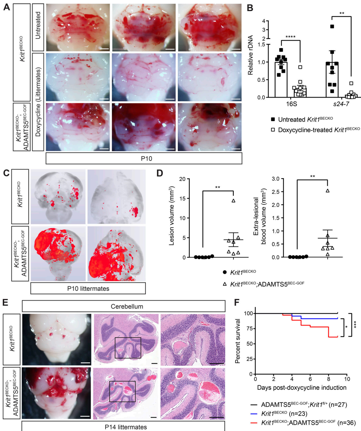
Figure 5. Endothelial gain of ADAMTS5 and loss of KRIT1 synergize during CCM formation. (A) Hindbrains from untreated Krit1 BECKO animals or doxycycline-treated Krit1 BECKO and Krit1 BECKO ; ADAMTS5 BEC-GOF littermate animals at P10. Images from three different doxycycline-treated litters are shown and representative of seven litters. Scale bars, 1 mm. (B) Relative quantification of neonatal gut bacterial load measured by qPCR of bacterial 16S and Bacteroidetes s24-7 rRNA gene copies ( n = 9 or 10 from at least three litters, Student's t test). (C) Composite microCT images from the hindbrain (left) and forebrain (right) of Krit1 BECKO and Krit1 BECKO ; ADAMTS5 BEC-GOF littermates. (D) Volumetric analysis of lesional and extra-lesional blood. The distinction between lesional and extra-lesional blood is shown due to the high rate of peri-lesional hemorrhage in Krit1 BECKO ; ADAMTS5 BEC-GOF animals compared with Krit1 BECKO animals ( n = 6 or 7 from six litters, Mann-Whitney U test). (E) Visual assessment (left) and corresponding H&E staining (center and right) of the hindbrain demonstrate an increase in both the size and number of CCM lesions in Krit1 BECKO ; ADAMTS5 BEC-GOF mice compared with Krit1 BECKO mice. Higher magnification images are shown on the right. Scale bars, 1.5 mm (white) and 250 \mu m (black). Results are representative of three litters. (F) Kaplan-Meier survival curves of ADAMTS5 BEC-GOF ; Krit1 fl/+ , Krit1 BECKO , and Krit1 BECKO ; ADAMTS5 BEC-GOF mice during the first 10 d of life following doxycycline induction at P1 ( n = 23 –36 per group from 19 litters, log-rank test). Error bars represent \pm SEM; *, P < 0.05 ; **, P < 0.01 ; ***, P < 0.001 ; ****, P < 0.0001 .
