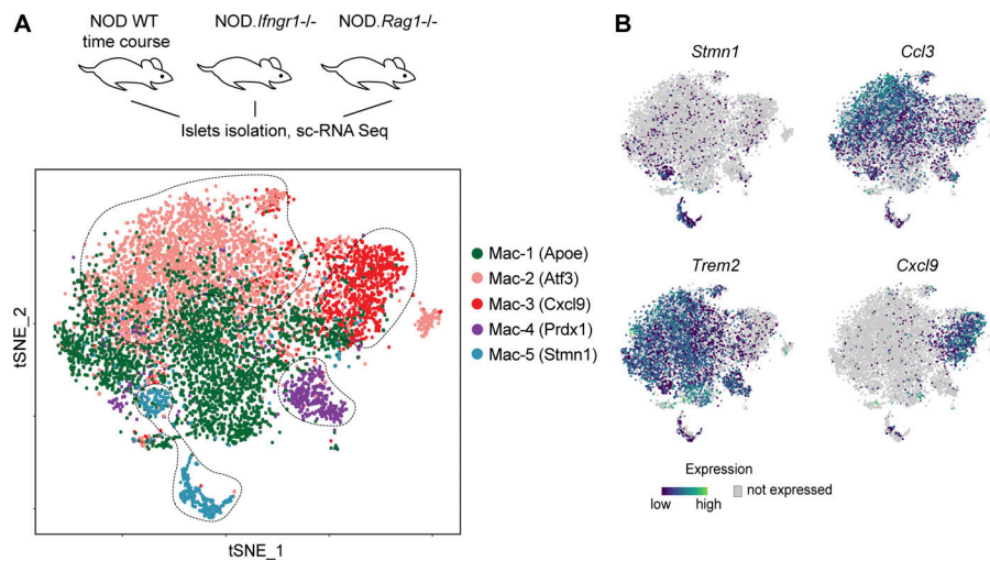
Figure S5. Characterization of NOD. Ifng1 -/- and NOD. Rag1 -/- samples. (A) t-SNE sc-RNaseq plot from the NOD macrophage time-course samples merged with two knockout samples: NOD. Ifng1 -/- (8 wk) and NOD. Rag1 -/- (8–16 wk). (B) Expression of the marker genes in the populations of the merged macrophage dataset.
