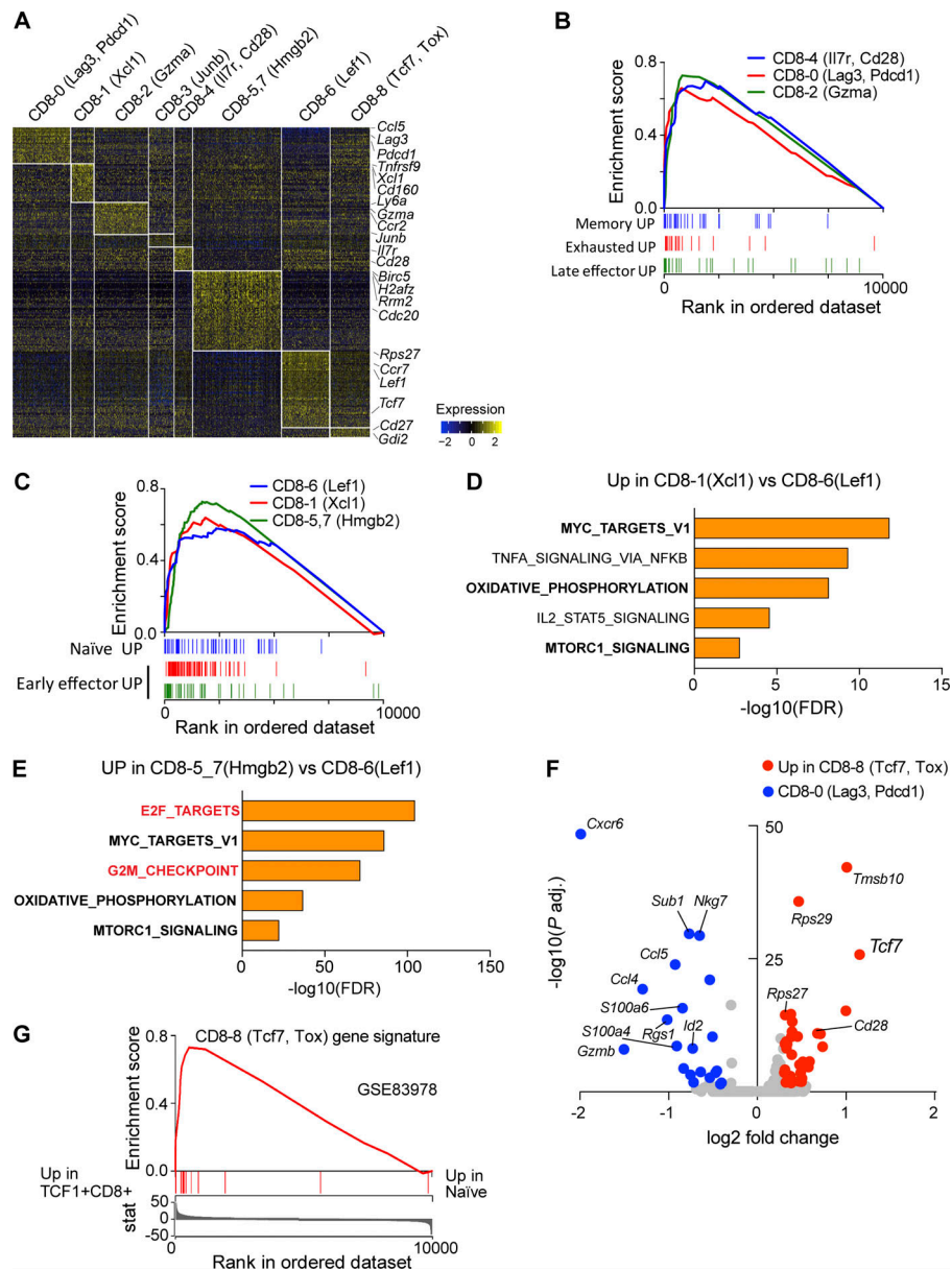
Figure S3. Islet CD8 T cell heterogeneity. (A) Heatmap of differentially expressed genes driving islet CD8 T cell heterogeneity (LFC > 0.3, adjusted P < 0.05 , Wilcoxon rank sum test with Benjamini–Hochberg correction). Cells were pooled from 4-, 8-, and 15-wk-old samples. (B and C) CD8 T cell transcriptional profile (GSE41867) was used as a reference dataset for CD8 T cell annotation (see Materials and methods; Table S5). GSEA plots showing population signatures correlated with different CD8 T cells phenotypes (all FDR < 0.01). (D and E) Hypergeometric pathway analysis (hallmark MSigDB database, Benjamini–Hochberg correction applied) on two early effector populations: CD8-1(Xcl1) (D) and CD8-5,7(Hmgb2) (E). Shared pathways are in bold; specific to CD8-5,7(Hmgb2) are in red. (F) Scatter plot shows differential gene expression between two exhausted T cell populations, CD8-8(Tcf7, Tox) and CD8-0(Lag3, Pdcd1), based on Wilcoxon rank sum test with Benjamini–Hochberg correction. Log N fold cutoff of 0.25 used. Genes of interest are labeled. (G) GSEA plot showing CD8-8(Tcf7, Lag3) signature enrichment into the dataset, comparing CD8 + TCF1 + (Tcf7 encoded) and naïve CD8 cells (GSE83978). FDR < 0.01.
