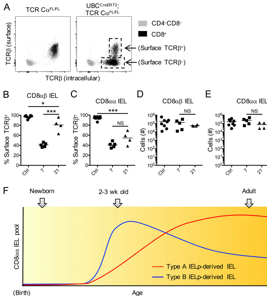
Figure 5. Reliance on TCR for IEL maintenance. (A) Representative plots of peripheral blood samples taken from TCR \text{C}\alpha^{\text{FL/FL}} (left plot, control) or UBC ^{\text{CreERT2}} TCR \text{C}\alpha^{\text{FL/FL}} mice (right plot) 7 d after administration of tamoxifen. The samples were surface stained for CD4 and CD8 and surface stained with one fluorochrome-conjugated antibody to TCR \beta , then intracellularly stained with another. Shown are CD4-CD8- cells (gray) and CD8+ T cells (black). (B-E) Frequency of surface TCR \beta^+ within total (surface and intracellular) TCR \beta^+ CD8 \alpha\beta IELs (B) or CD8 \alpha\alpha IELs (C) and numbers of total CD8 \alpha\beta IELs (D) and CD8 \alpha\alpha IELs (E) in the small intestine of TCR \text{C}\alpha^{\text{FL/FL}} (control) and UBC ^{\text{CreERT2}} TCR \text{C}\alpha^{\text{FL/FL}} (sample) mice. (F) Proposed model for CD8 \alpha\alpha IEL establishment. Each symbol in B-E represents an individual mouse. Horizontal lines indicate the mean. Data are pooled from eight independent experiments. * P < 0.05 and *** P < 0.001 (ANOVA with Bonferroni post-test).
