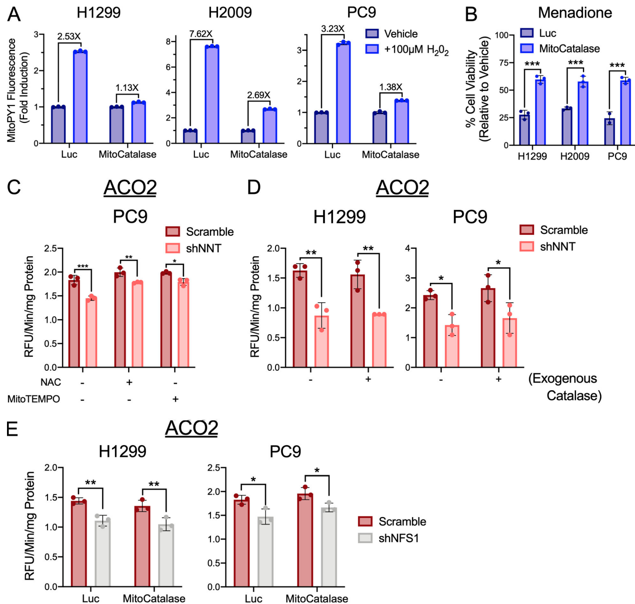
Figure S5. MitoCatalase protects against mitochondrial oxidation. (A) Fold inductions of MitoPY1 fluorescence in Luc or MitoCatalase-expressing NSCLC cells challenged with 100 \mu M H_2O_2 . (B) Viability of Luc or MitoCatalase expressing NSCLC cells following 24 h treatment with 15 \mu M (H1299) or 25 \mu M (H2009, PC9) menadione (Student's t test). Cell viability was determined relative to vehicle-treated controls. (C) Average ACO2 activity in mitochondrial lysates of PC9 cells subject to scramble or shNNT lentiviral infection following a 24-h treatment with vehicle (0.05% DMSO), 1 mM NAC, or 25 nM MitoTEMPO (two-way ANOVA). (D) Average ACO2 activity in mitochondrial lysates of NSCLC cells subject to scramble or shNNT lentiviral infection following an overnight treatment with 1,000 U of recombinant catalase (two-way ANOVA). (E) Average ACO2 activity in mitochondrial lysates of Luc or MitoCatalase-expressing NSCLC cells following NFS1 knockdown (two-way ANOVA). Data are representative of one experiment of three experimental replicates. Data are represented as mean \pm SD of three technical replicates. *, P < 0.05 ; **, P < 0.01 ; ***, P < 0.001 .
