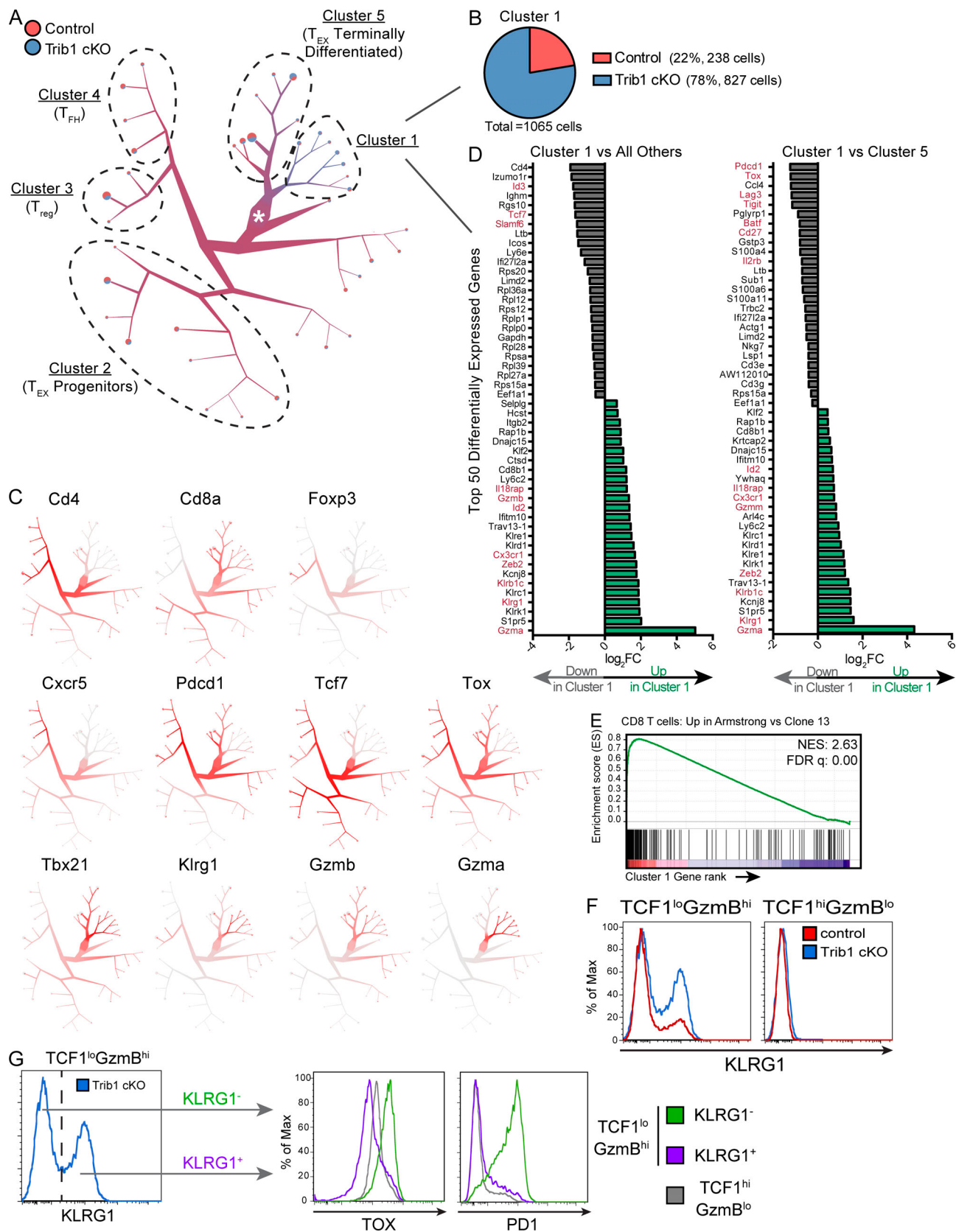
Figure 6. scRNA-seq analysis reveals a KLRG1 + effector population that is transcriptionally distinct from T_{EX} subsets and is enriched in the absence of Trib1. Activated T cells ( TCR\beta^+CD44^+ ) were isolated by FACS from spleens of either control or Trib1 cKO mice at day 15 after clone 13 infection and prepared for scRNA-seq analyses. (A) Visualization of single-cell clustering using TooManyCells from 7,611 TCR\beta^+CD44^+ cells. All cells begin at the central node (white star) and are recursively bipartitioned based on transcriptional similarity. To this end, TooManyCells produces a hierarchy of nested cell clusters where each
