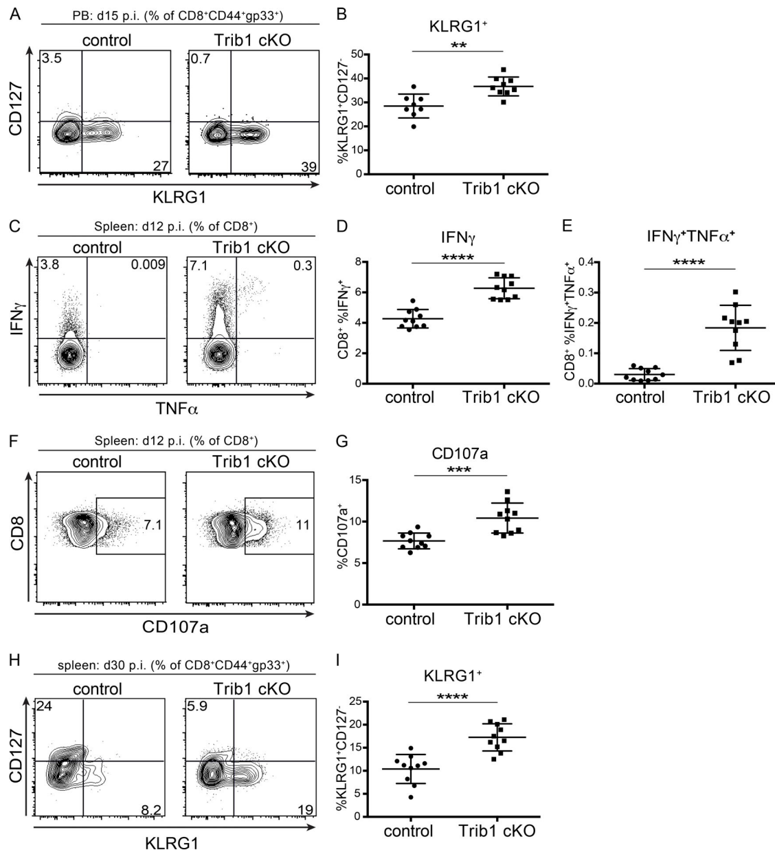
Figure S3. Trib1 deficiency promotes D 8 GP33 + T cell effector-like responses in chronic infection. (A and B) Representative flow plots (A) and summary of the frequency of peripheral blood (PB) LCMV-specific CD8 effector-like T cells (KLRG1 + CD127 - , gated on CD8 + CD44 + gp33 + ) at day 15 after clone 13 infection (B). (C–E) Representative flow plots (C) and summary of cytokine production in splenic CD8 T cells harvested from mice at day 12 p.i. and stimulated ex vivo with gp33 peptide for 5 h (D and E). (F and G) Representative flow plots (F) and summary of CD107a staining in splenic CD8 T cells harvested from mice at day 12 p.i. and stimulated ex vivo with gp33 peptide for 5 h (G). (H and I) Representative flow plots (H) and summary of the frequency of splenic LCMV-specific CD8 effector-like T cells (KLRG1 + CD127 - , gated on CD8 + CD44 + gp33 + ) at day 30 after clone 13 infection (I). Data in A and B are representative of three independent experiments with 7–10 mice per genotype. Data in C–G are representative of two independent experiments each with 7–10 mice per genotype. Data in H and I are representative of three independent experiments each with 8–10 mice per genotype. Error bars are mean \pm SD. **, P < 0.01 ; ***, P < 0.001 ; ****, P < 0.0001 by unpaired Student's t test. Control: CD4-cre + Trib1 +/+ ; Trib1 cKO: CD4-cre + Trib1 F/F .
