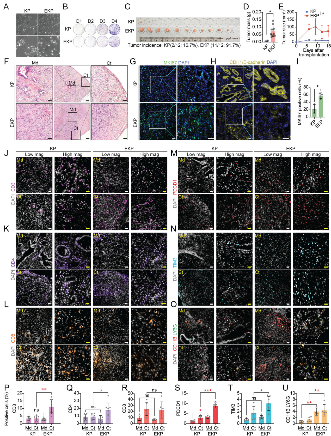
Figure 4. Cdh1 KO promotes KP-driven gastric tumorigenesis. (A) Bright-field images of KP and EKP cells in low and high magnification. Scale bars: 100 \mu m (upper panels); 50 \mu m (lower panels). (B) Crystal violet staining of KP and EKP GOs-derived cells. (C) Bright-field images of KP and EKP allograft tumors; tumor incidence of allograft tumors. (D and E) Plot for tumor mass (D) and tumor size (E) assessment of KP and EKP allografts. (F) H&E staining of KP and EKP allograft tumors ( n \geq 3 ). Scale bars (from left to right): 50, 200, 50 \mu m; Md: middle; Ct: cortex. (G and H) Immunostaining of KP and EKP allograft tumors ( n \geq 3 )
