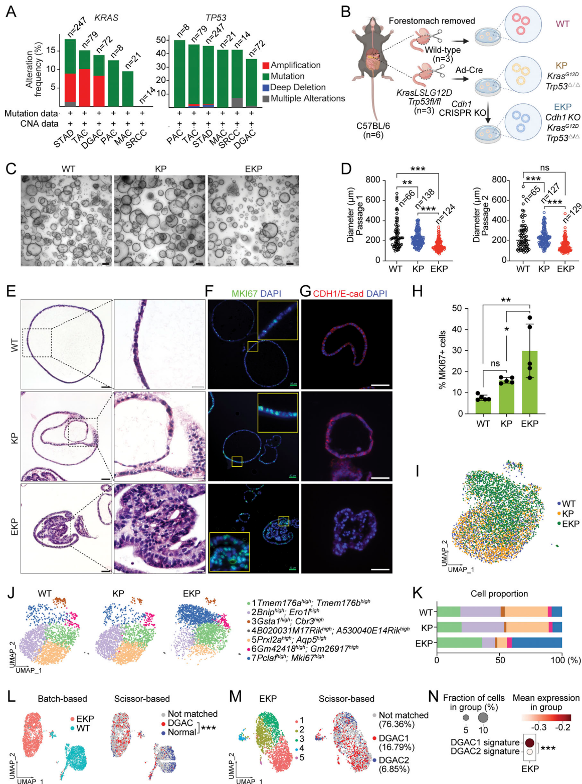
Figure 3. Establishment of genetically engineered gastric organoids with Cdh1 -inactivation. (A) Genetic alteration of the KRAS and TP53 genes based on the cBioPortal. n represents the total number of patients enrolled in each subtype. DGAC, diffuse-type gastric adenocarcinoma; SRCC, signet ring cell carcinoma; TAC, tubular adenocarcinoma; STAD, stomach adenocarcinoma; MAC, mucinous adenocarcinoma; PAC, papillary adenocarcinoma. (B) Illustration of the workflow for stomach tissue collection and dissociation, gene manipulation of the gastric organoids (GOs), GOs culture, and representative image of GOs. Three GO lines were generated, including WT, KP, and EKP. WT mice and KP mice were sacrificed to collect stomach tissue. After removing the forestomach, stomach tissue was dissociated into a single cell and culture as organoids. Adeno-Cre virus was used to treat Kras LSL-G12D ; Trp53 fl/fl organoids to generate KP organoids, followed by nutlin-3 selection. After selection, EKP organoids were generated using CRISPR-mediated Cdh1 KO from KP GOs. (C) Representative images of WT, KP, and EKP GOs at passage day 8. Scale bars: 200 \mu m. (D) Growth analysis for WT, KP, and EKP GOs in two passages on day 8 of each passage.
