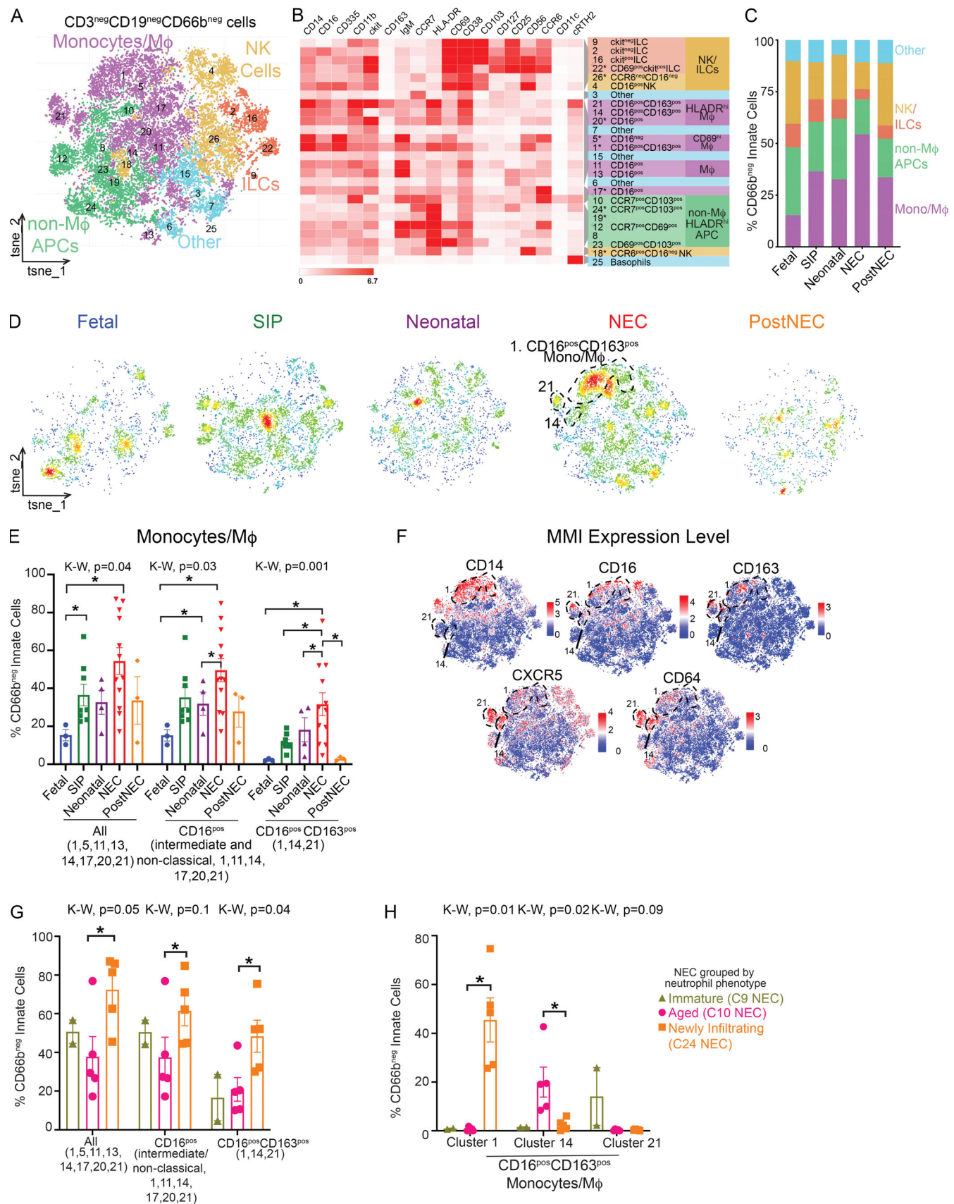
Figure 2. Monocytes expressing CD16 and CD163 are enriched in NEC mucosa. (A) tSNE plot of CD3 neg CD19 neg CD66b neg cells. (B) Clustergram (Fernandez et al., 2017) heatmap of canonical surface markers used to identify populations in each cluster; colors correspond to A. Asterisks denote clusters with significant
