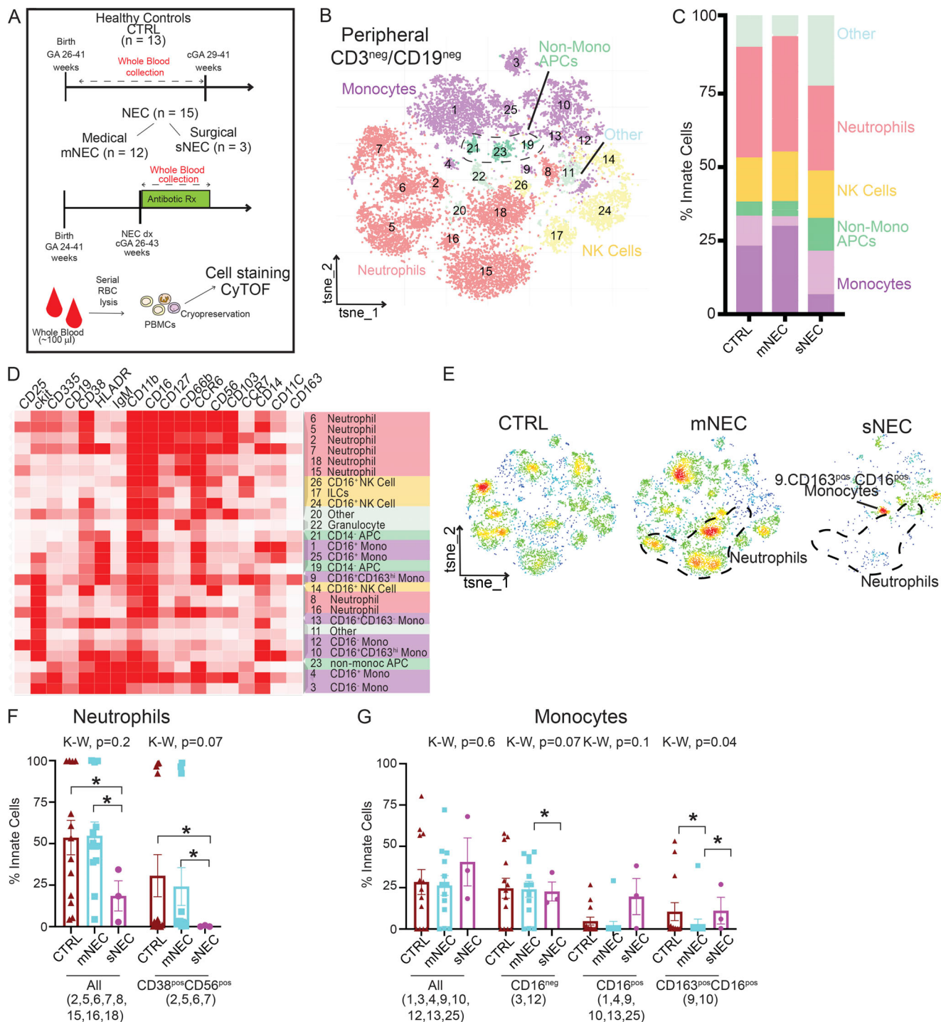
Figure 3. Peripheral neutropenia and increase in CD16 + CD163 + monocytes/Mφ in infants with surgical NEC. (A) Workflow for collection and analysis of peripheral blood. (B) tSNE of peripheral CD3 neg CD19 neg innate cells. (C) Abundance of major populations expressed as a percentage of innate cells. (D) Clustergram (Fernandez et al., 2017) of median expression of canonical markers used to identify individual clusters. (E) Density tSNE plots of each group. (F and G) Neutrophils (F) and monocytes (G) expressed as a percentage of circulating innate cells. Each dot represents one patient. Box plots represent mean ± SE. *, P < 0.05. cGA, corrected GA; dx, diagnosis; K-W, Kruskal-Wallis test.
