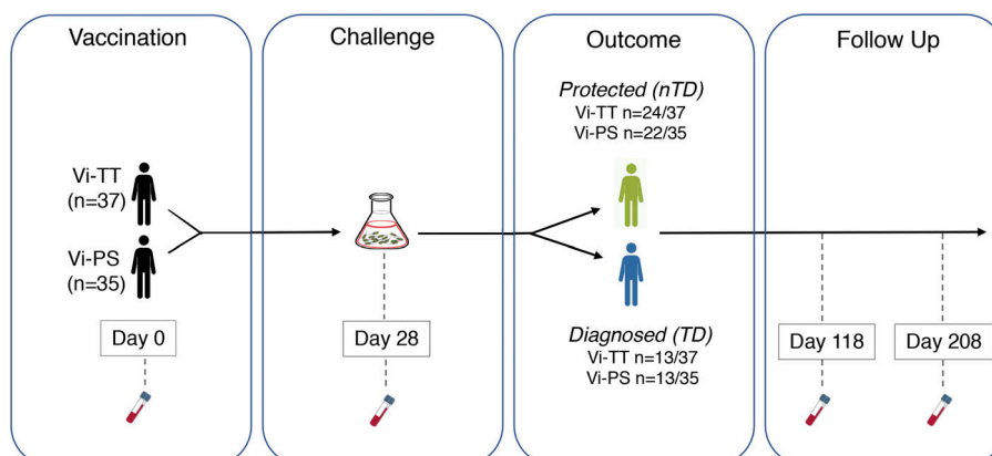
Figure 1. Schematic of S. Typhi CHIM study design. Participants were randomized, vaccinated with Vi-TT ( n = 37 ) or Vi-PS ( n = 35 ), orally challenged with live S. Typhi bacteria on day 28. Participants were monitored over a 14-day challenge period. Individuals with S. Typhi bacteremia or persistent fever ( \geq 38^\circ\text{C} for \geq 12 h) were diagnosed with typhoid fever (TD; Vi-TT, n = 13/37 ; Vi-PS, n = 13/35 ). Participants who did not meet the diagnostic criteria for typhoid fever were classified as nTD (Vi-TT, n = 24/37 ; Vi-PS, n = 22/35 ). Vi-specific humoral responses were evaluated on day 0 (before vaccination) and days 28, 118, and 208.
