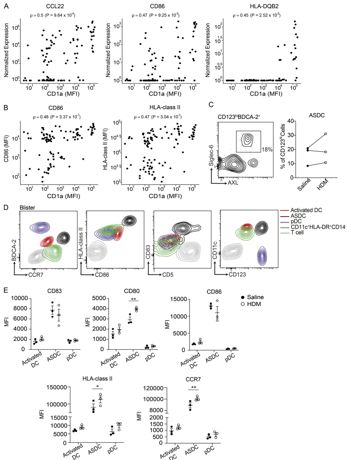
Figure 4. Human skin activated DCs and ASDCs express genes and proteins relating to antigen presentation. (A) CD1a protein expression is significantly correlated with gene expression of CCL22 ( \rho = 0.5 , P < 0.05 ), CD86 ( \rho = 0.47 , P < 0.05 ), and HLA-DQB2 ( \rho = 0.45 , P < 0.05 ). Each dot represents an individual cell. Spearman correlation was performed. (B) Flow cytometry of CD1a, CD86, and HLA class II expression of BDCA-2 + DCs from skin suction blisters. Correlations between CD86 and CD1a ( \rho = 0.48 , P < 0.05 ) and HLA-DR and CD1a ( \rho = 0.47 , P < 0.05 ) are shown. Each dot represents an individual cell. Spearman correlation was performed. One representative result of three independent experiments is shown. (C–E) Mononuclear cells isolated from skin suction blisters were analyzed for DC subsets by flow cytometry. The percentage of ASDCs (C) and expression of BDCA-2, CCR7, HLA class II, CD86, CD83, CD123, and CD11c of activated DCs (red), ASDCs (black), bona fide pDCs (purple), cDCs (green), and T cells (gray) in the saline- and HDM-challenged blisters (D and E) are shown. One representative result of two independent experiments is shown; each dot represents a donor. One to two blisters per challenge condition were created per upper arm of each donor. MFI, mean fluorescence intensity. Lines represent the mean + SEM. *, P < 0.05 ; **, P < 0.01 ; Student's t test or two-way ANOVA.
