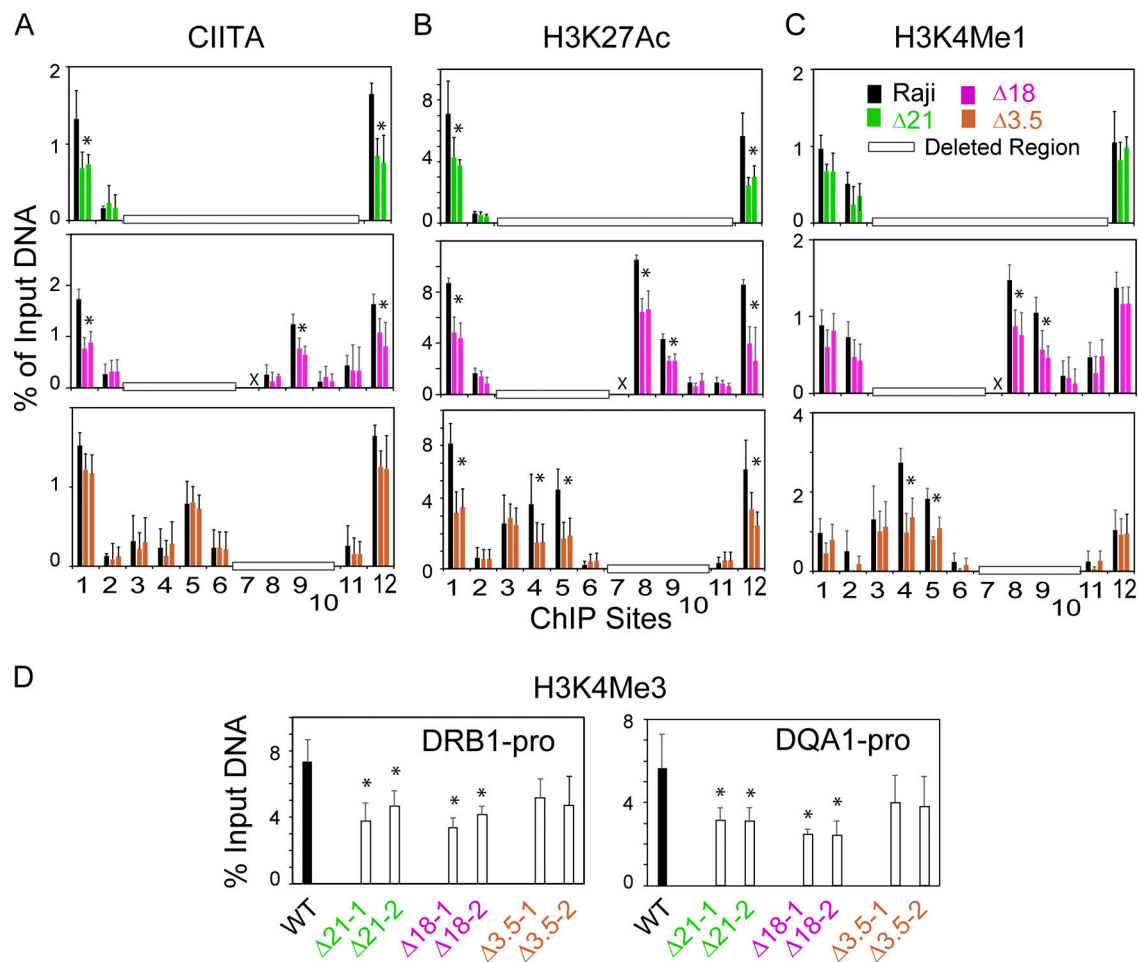
Figure 5. CIITA recruitment and histone modifications are altered at MHC-II promoters following deletion of DR/DQ-SE . (A–C) Conventional ChIP-qPCR assays for binding of CIITA or enrichment (A) of H3K27ac (B) and H3K4me1 (C) were performed on Raji (WT) or two represented isolates for each of the mutations deleting the DR/DQ-SE ( \Delta 18 ), XL9-SE ( \Delta 3.5 ), or both ( \Delta 21 ) regions. Positions of ChIP PCR sites 1–12 are shown in Fig. 1 A. (D) ChIP assays for H3K4me3 were performed at the indicated promoter regions. ChIP assays were performed in triplicate from three independent cultures. X represents ChIP assays not performed for the indicated site. Horizontal open bars represents ChIP sites deleted in the mutants assayed. Data represent mean \pm SD. For A–C, Student's t tests were performed to determine the significance between a WT sample and a mutant sample. For D, a one-way ANOVA with Tukey's post hoc test was performed to assess significance. *, P \leq 0.05 .
