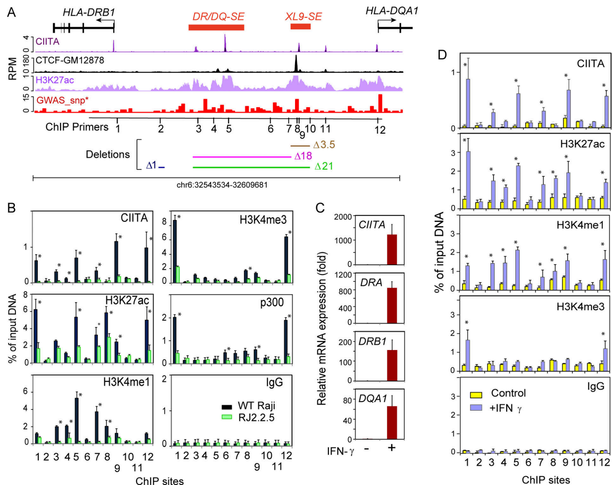
Figure 1. Two SEs reside in the intergenic region between HLA-DRB1 and HLA-DQA1 . (A) Schematic of the HLA-DR, -DQ intergenic region. CIITA, CTCF, and H3K27ac ChIP-seq data from The ENCODE Project Consortium (2012) and Scharer et al. (2015) are plotted with respect to the HLA-DRB1 and HLA-DQA1 genes. Red bars represent the DR/DQ-SE and XL9-SE SEs. The GWAS-SNP track shows the density of disease-associated SNPs in 500-bp bins across the region. The positions of ChIP primers (Table S1) are shown, as are regions that are deleted in the CRISPR/Cas9 mutant series. (B) Conventional ChIP-qPCR was performed on Raji and RJ2.2.5 cell chromatin for the indicated antibody with ChIP primer sets located at positions illustrated in A. (C) Relative fold change of the indicated gene expression as determined by qRT-PCR of A-431 cells \pm 24 h treatment with IFN \gamma . (D) ChIP as in B of A-431 cells \pm IFN \gamma treatment. Experiments in this figure were performed at least three times from independent cultures. Data represent mean \pm SD, and significance was determined by Student's t tests. *, P \leq 0.05.
