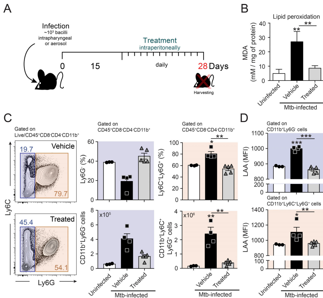
Figure 5. Lipid peroxidation induced by Mtb in vivo is inhibited by Fer-1 treatment. (A–D) C57BL/6 mice were infected by intrapharyngeal inoculation with \sim 10^3 bacilli of Mtb (H37Rv) as a model of severe TB and the animals sacrificed at 28 d p.i. Infected mice were treated daily by intraperitoneal injection with vehicle or Fer-1 (3 mg/kg/body weight) starting on day 15 p.i. ( n = 4 –5). (A) Schematic presentation of the experimental protocol. (B) Lipid peroxidation (malondialdehyde) measured in lung homogenates from uninfected and Mtb-infected mice. (C) Sample FACS plot and summary data of frequency and cell numbers of monocyte/macrophage (CD11b + Ly6C - ) and neutrophil subsets (CD11b + Ly6C + Ly6G + ) in the lungs. (D) Lipid peroxidation in monocyte/macrophage (CD11b + Ly6C - ) and neutrophil subsets (CD11b + Ly6C + Ly6G + ) in the lungs analyzed by flow cytometry. The data shown represent the means \pm SEM of four to five samples per experiment. Significant differences are indicated with asterisks (*, P < 0.05 ; **, P < 0.01 ; ***, P < 0.001 ). The data shown are representative of three separate experiments performed.
