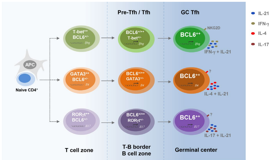
Model of IFN- \gamma -producing Tfh cell differentiation. In the T cell zone, once naive CD4 T cell is activated, T-bet is transiently expressed by a subset of BCL-6 +/- cells. T-bet is then down-regulated by BCL-6 when it migrates into the B cell zone and GC and differentiates into mature Tfh cells. These ex-Tbet Tfh cells have the capability to produce IFN- \gamma in addition to IL-21 and highly express cell surface protein NKG2D. As a general hypothesis, transient induction of T-bet, GATA3, or RORyt during Tfh cell differentiation may determine the generation of IFN- \gamma -, IL-4-, or IL-17-producing Tfh cell subsets. However, generalization of this model requires future development of new genetic tools, including mouse strains carrying inducible Cre driven by the Gata3 or Rorc locus.
