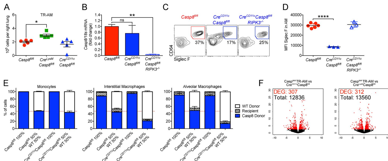
Figure 3. TR-AMs in LysM Cre Casp8 flox/flox and CD11c Cre Casp8 flox/flox mice have preserved expression of Casp8 , suggesting they escape Cre-mediated recombination. (A) CD11c Cre Casp8 flox/flox and LysM Cre Casp8 flox/flox mice have a normal number of TR-AMs in a steady state ( n = 5 mice per group; data are shown as mean \pm SEM; one-way ANOVA with Dunnett's test for multiple comparisons; *, P < 0.05 ; the experiment was performed three times). (B) Casp8 expression in flow-sorted TR-AMs measured by quantitative PCR ( n = 3 –5 mice per group; data are shown as mean \pm SEM; one-way ANOVA with Dunnett's test for multiple comparisons; **, P < 0.01 ; the experiment was performed two times). (C and D) Bone marrow from CD11c Cre Casp8 flox/flox mice fails to reconstitute the alveolar niche 8 wk after irradiation, as indicated by ongoing recruitment of the immature Mo-AMs with low expression of Siglec F. Repopulation of the alveolar niche was rescued in CD11c Cre Casp8 flox/flox RIPK3 -/- mice ( n = 4 –5 mice per group; data are expressed as mean \pm SEM; one-way ANOVA with Dunnett's test for multiple comparisons; ****, P < 0.0001 ). (E) Alveolar macrophages derived from bone marrow from CD11c Cre Casp8 flox/flox mice fail to reconstitute the alveolar niche 8 wk after irradiation, as shown by decreased expression of Siglec F on alveolar macrophages. Mice were lethally irradiated, followed by reconstitution with bone marrow from control mice ( Casp8 flox/flox ) or bone marrow from mice with deletion of Casp8 in cells expressing CD11c ( Cre CD11c Casp8 flox/flox ), either alone or in combination with bone marrow from wild-type mice (50% mixture of the two genotypes). Monocytes, interstitial macrophages, and alveolar macrophages were identified by flow cytometry of lung homogenates 8 wk later (CD45.1 or CD45.2 mice were used for lineage tracing). Although ~50% of monocytes in both Casp8 flox/flox and Cre CD11c Casp8 flox/flox mice were wild-type cells, the majority of interstitial macrophages and alveolar macrophages in mice reconstituted with Cre CD11c Casp8 flox/flox bone marrow, but not Casp8 flox/flox mice, were of wild-type origin, suggesting the loss of Casp8 during differentiation results in a selective disadvantage in the differentiation of monocytes in to alveolar macrophages; data are shown as mean \pm SEM. (F) Cells that escaped Cre-mediated recombination behave similarly to wild-type cells during fibrosis (day 14) with <1% differentially expressed genes (DEG). Volcano plot showing number of differentially expressed genes (red, FDR q value < 0.05, n = 2 –5 mice per group).
