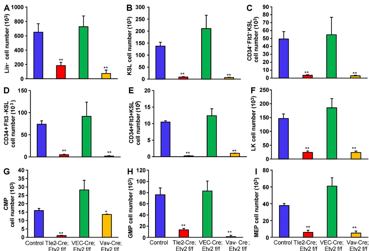
Figure 3. Hematopoietic but not endothelial deletion of Etv2 impairs HSPC recovery after 5-FU treatment. (A–I) Tie2-Cre; Etv2 CKO, VEC-Cre; Etv2 CKO, Vav-Cre; Etv2 CKO, or littermate control mice were injected with 250 mg/kg 5-FU i.p. After 11 d, BM mononuclear cells were subjected to flow cytometry by using HSPC surface markers to determine absolute cell number (per femur and tibia) of different hematopoietic compartments. (A) Lin - cells. (B) KSL (c-Kit + Sca1 + Lin - ) cells. (C) Long-term HSCs (CD34 - Flt3 - KSL). (D) Short-term HSCs (CD34 + Flt3 - KSL). (E) Multipotent progenitor (CD34 + Flt3 + KSL) cells. (F) LK (c-Kit + Sca1 + Lin - ) cells. (G) Common myeloid progenitor (CMP; CD34 + CD16/32 - LK) cells. (H) Granulocyte-macrophage progenitor (GMP; CD34 + CD16/32 + LK) cells. (I) Megakaryocyte-erythrocyte progenitor (MEP; CD34 - CD16/32 - LK) cells. n = 4–6 from two independent experiments. *, P < 0.05; **, P < 0.001. Error bars indicate standard error of the mean.
