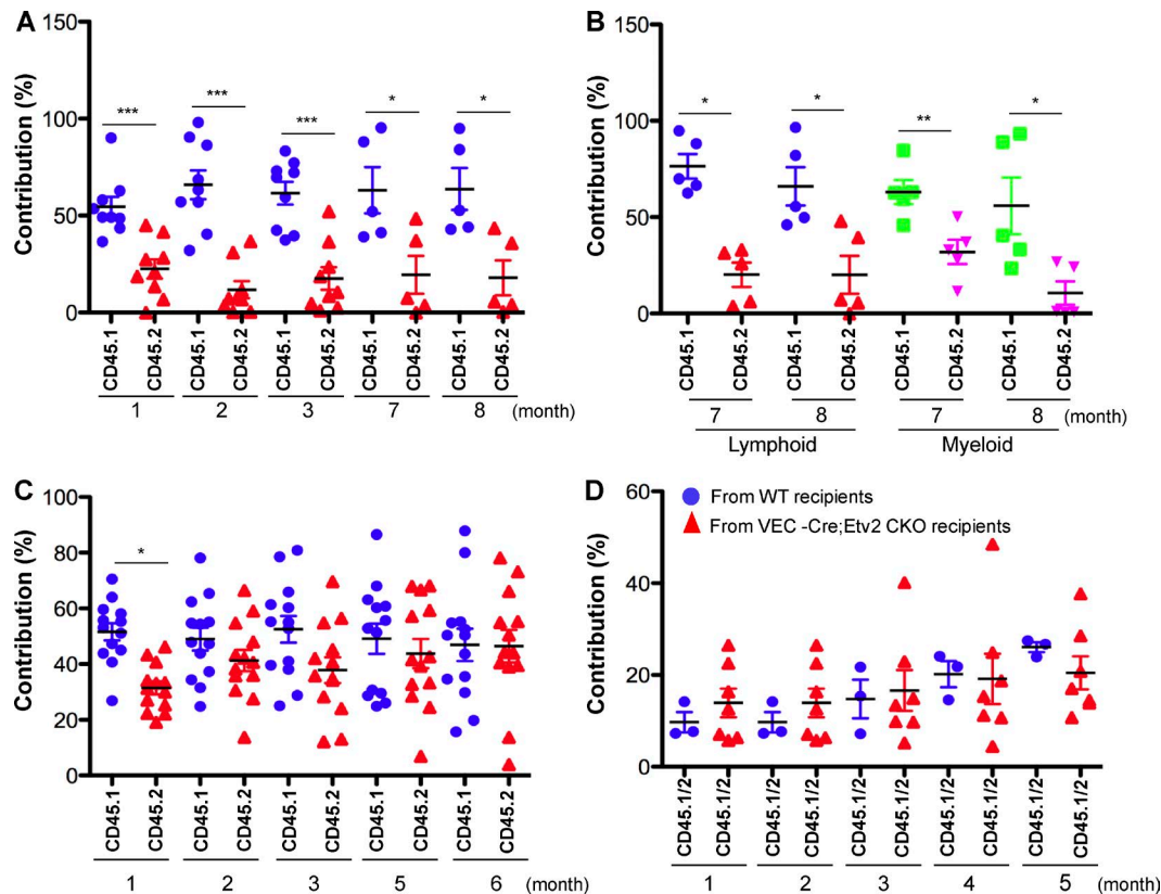
Figure 4. Hematopoietic but not endothelial deletion of Etv2 results in decreased hematopoietic reconstitution capacity. (A and B) 10,000 KSL cells from Vav-Cre; Etv2 CKO or littermate control mice (both are CD45.2) were transplanted along with 10^6 competitor BM cells (CD45.1) into lethally irradiated WT recipient mice (CD45.1 \times CD45.2). PB from recipients was analyzed for donor-derived contribution by determining the percentage of CD45.1 + and CD45.2 + PB leukocyte or lymphoid (B220 + /CD3 + or myeloid Gr1 + ) at the indicated time points after transplantation. n = 5-8 from two independent transplantations. (C) 10^6 BM cells from VEC-Cre; Etv2 CKO or littermate control mice (both are CD45.2) were transplanted along with 10^6 competitor BM cells (CD45.1) into lethally irradiated WT recipient mice (CD45.1 \times CD45.2). PB from recipients was analyzed for donor-derived contribution by determining the percentage of CD45.1 + and CD45.2 + PB leukocytes at the indicated time points after transplantation. n = 10-13 from three independent transplantations. (D) 2 \times 10^6 WT BM cells (CD45.1 \times CD45.2) were transplanted into lethally irradiated WT or VEC-Cre; Etv2 CKO recipients (both are CD45.2). 6 mo after transplantation, 2 \times 10^6 BM cells (CD45.1 \times CD45.2) recovered from WT or VEC-Cre; Etv2 CKO recipients were transplanted along with 5 \times 10^5 competitor BM cells (CD45.1) into lethally irradiated recipient mice (CD45.2). PB was analyzed for donor-derived contribution by determining the percentage of CD45.1 + CD45.2 + PB leukocytes at the indicated time points after transplantation. n = 3-6 from two independent experiments. *, P < 0.05 ; **, P < 0.01 ; ***, P < 0.001 .
