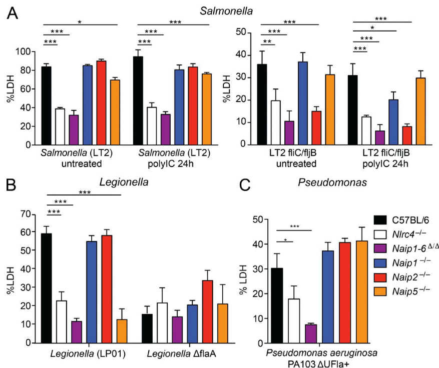
Figure 3. Requirement for individual NAIPs for pyroptosis during macrophage infection. (A–C) LDH release assay of supernatants of WT, Nlrc4 -/- , Naip1 -6 ΔΔ , Naip1 -/- , Naip2 -/- , and Naip5 -/- BMMs infected with WT LT2 or flagellin-deficient ( fljC fljB ) S. Typhimurium (MOI = 5) for 6 h, with or without 5 μg/ml polyIC 24 h before infection (note different y-axis scales for WT and flagellin-deficient data; A), WT LP02 or flagellin-deficient L. pneumophila (MOI = 5) for 4 h (B), or P. aeruginosa (MOI = 20) PA103ΔU Fla + for 2 h after 3-h pretreatment with 50 ng/ml LPS (C). Data are representative of two independent experiments ( n = 3), mean ± SD; one-way ANOVA, Dunnett's post test: *, P < 0.05; **, P < 0.01; ***, P < 0.001.
