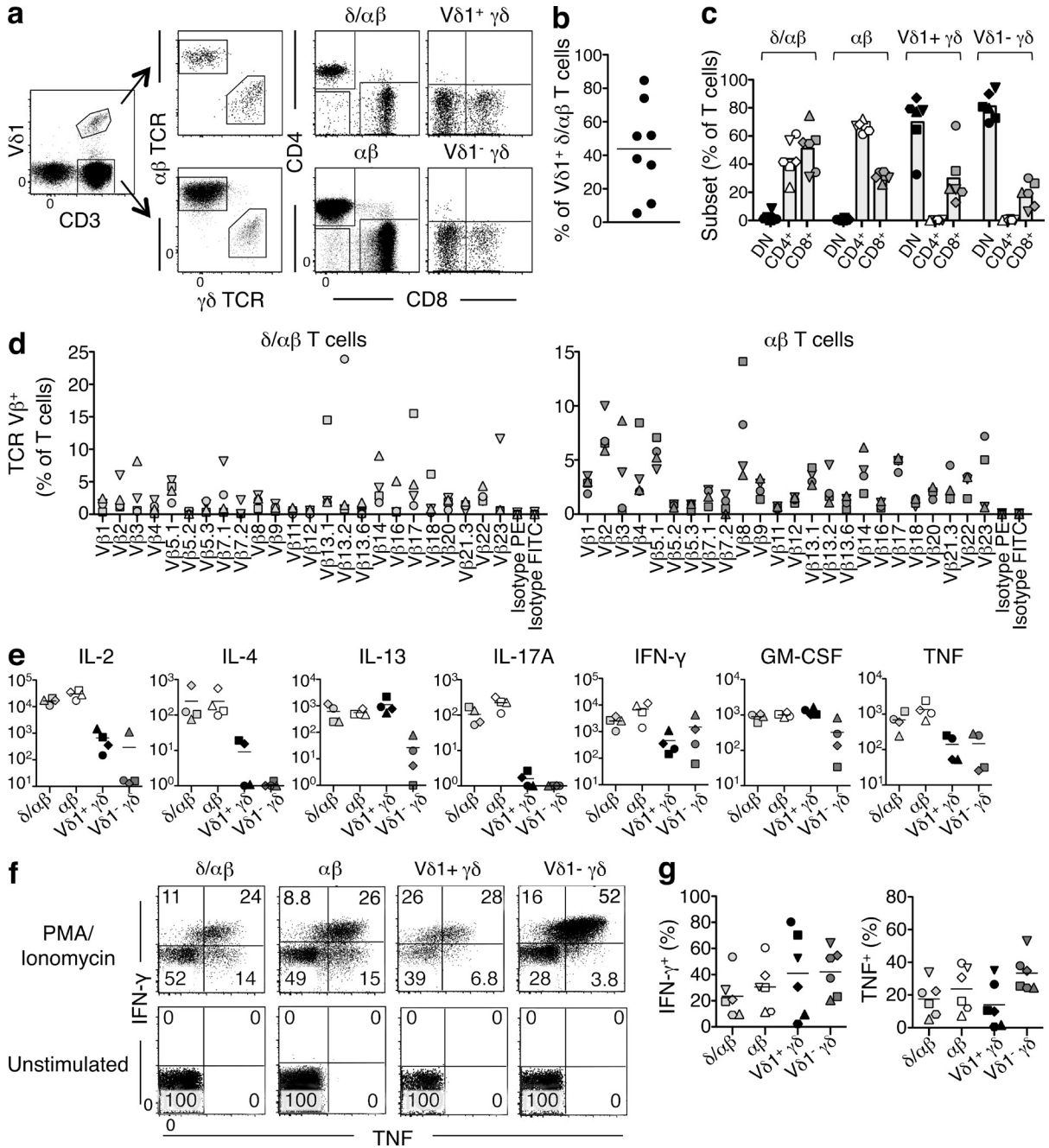
Figure 3. TCR-Vδ1 + cells consist of γδTCR + and δ/αβTCR + subsets. (a) CD14 - CD19 - lymphocytes from a representative healthy blood donor, were analyzed by flow cytometry. Plots show CD3 + Vδ1 + and CD3 + Vδ1 - PBMC subsets, gated as indicated (left plot), and then subsets labeled with anti-αβTCR (identifying δ/αβ T cells and αβ T cells) versus anti-γδTCR (identifying γδ T cells) are shown (second plots). Expression of CD4 and CD8 on these subsets is also shown (right-hand plots). (b) The percentage of Vδ1 + cells that were αβTCR + (i.e., δ/αβ T cells) was calculated for eight donors using the gating strategy shown in a. (c) The percentage of CD4 - CD8 - (double negative [DN]), CD4 + CD8 - (CD4 + ), and CD4 - CD8 + (CD8 + ) cells within Vδ1 + αβTCR + (δ/αβ), Vδ1 - αβTCR + (αβ), Vδ1 + γδTCR + (Vδ1 + γδ), and Vδ1 - γδTCR + (Vδ1 - γδ) is shown, with each symbol representing a separate donor ( n = 6) and bar graphs depicting the mean value. (d) Healthy human PBMCs were stained with a panel of anti-TCR-Vβ-specific antibodies. Plots show the percentage of Vδ1 + αβTCR + (δ/αβ, left) and Vδ1 - αβTCR + (αβ, right) T cells that bound to each Vβ antibody. Graphs depict n = 4 donors with each symbol representing a different donor. (e) δ/αβ T cells, αβ T cells, Vδ1 + γδ T cells, and Vδ1 - γδ T cells (as defined in c) were purified by FACS and stimulated with anti-CD3/CD28 beads for 72 h. Cytokines in culture supernatants were measured by cytometric bead array. Each data point represents the mean of n = 2–4 replicates from one donor, with n = 4 donors and each symbol shape representing a different donor. (f) δ/αβ, αβ, Vδ1 + γδ, and Vδ1 - γδ T cells from a representative donor (as defined in c) were stimulated for 4 h with PMA/ionomycin (top plots) or unstimulated (bottom plots), and IFN-γ and TNF were measured by intracellular cytokine staining. (g) Percentage of IFN-γ- and TNF-producing cells stimulated as in e, with each symbol representing a separate donor ( n = 6). Symbols indicating specific donors within panels do not correlate with the same donors between different panels. (b, e, and g) Horizontal lines indicate the mean.
