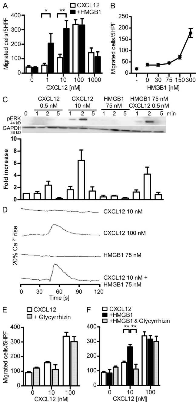
Figure 2. HMGB1 increases CXCL12-induced activities in human monocytes and CXCR4-transfected cells and is sensitive to glycyrrhizin. (A) Chemotaxis toward increasing concentrations of CXCL12 ± 300 nM HMGB1. Migrated cells were counted per five high-power fields (HPF) and are shown as mean ± SEM of three independent experiments performed with cells from different donors (*, P < 0.05; **, P < 0.01, ANOVA plus Bonferroni posttest). (B) Dose-response curve of HMGB1 in the presence of 10 nM CXCL12. Migrated cells were counted per five high-power fields and are shown as mean ± SEM of three independent experiments. (C) Time course of ERK1&2 phosphorylation induced by CXCL12 alone or in the presence of HMGB1. The intensity of pERK1&2 bands was analyzed by densitometry, normalized with matching GAPDH, and compared with the unstimulated control. One representative blot is shown; the bars and error bars represent mean ± SEM of four independent experiments with
