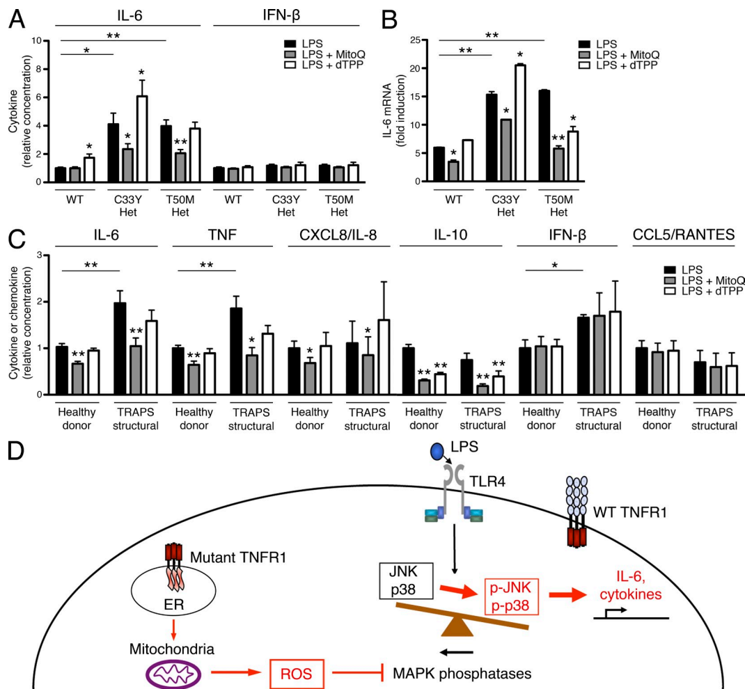
Figure 7. Inhibition of mitochondrial ROS can reduce normal cytokine production and reverse hyperinflammatory responses in TRAPS.
