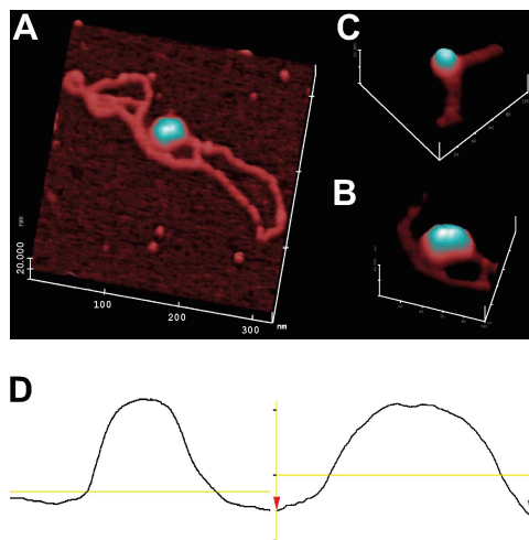
Figure 3. AFM of pKMP2 plasmids with nucleosomes. (A) Full-length plasmid (DNA contour length measured to be ~1.1 \mu m or ~3.2 kb). The magnification is 200,000 \times , with a 20-nm full-scale z axis. Using the AFM offline software, the full contour length of the free DNA was segmented into ~50 linear segments, each ~20 nm in length, and the segment lengths were tallied. (B) Portion of another pKMP2 plasmid with a single nucleosome. The magnification is 300,000 \times , with a 10-nm full-scale z axis. (C) The magnification is 300,000 \times , with a 10-nm full-scale z axis of a portion of the plasmid shown in A. (D) Single-line topographic AFM traces of the mononucleosome (left) and dinucleosome (right) as shown in B and C, respectively. The trace of the dinucleosome shows a bipartite topography and is roughly twice the size of the mononucleosome. The experiment was done twice with similar results.
