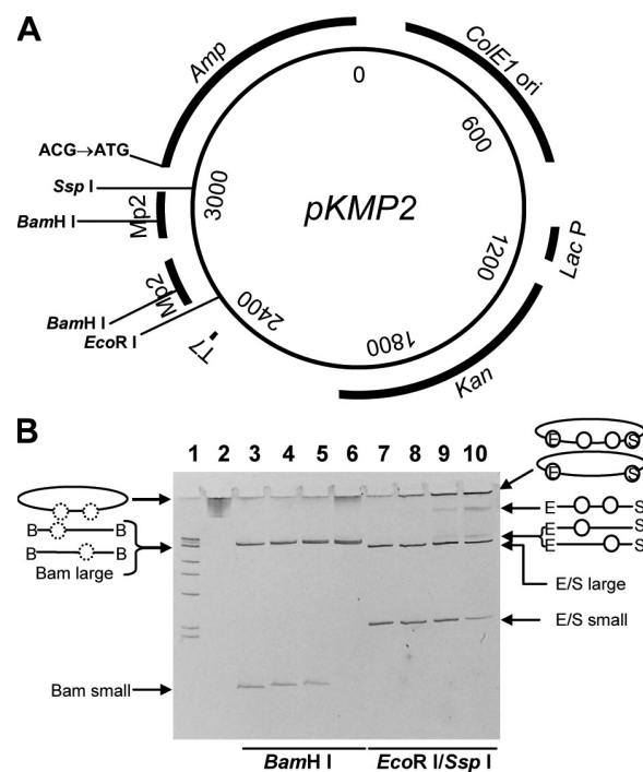
Figure 1. The pKMP2 plasmid and its charging with nucleosomes.
