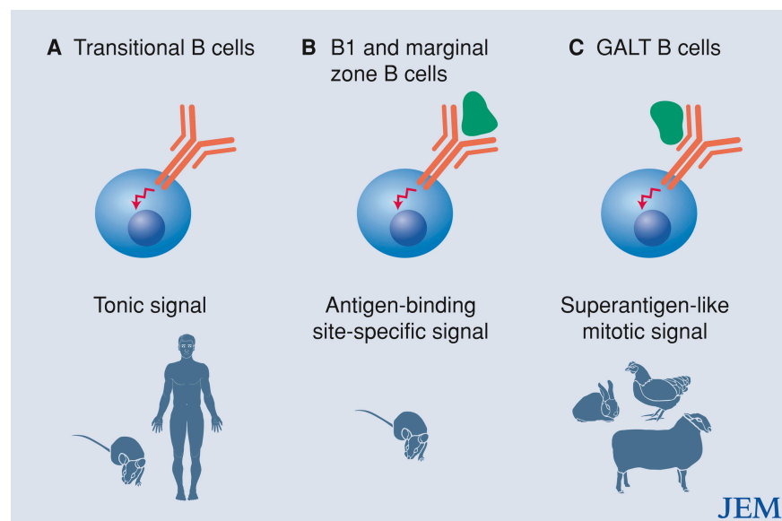
Figure 1. Different modes of BCR signaling are referred to as positive selection. (A) A constitutive tonic signal through the BCR and the Ig\alpha - Ig\beta complex. (B) An authentic antigen binding site-specific signal. (C) A superantigen-like signal that acts through binding of framework residues in the V regions. Examples of B cell subsets in which such type of positive selection takes place are shown.
