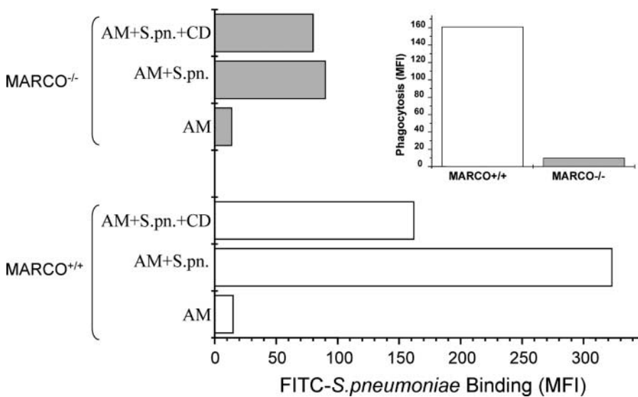
Figure 3. Binding and phagocytosis of FITC-labeled S. pneumoniae (S.pn.) by MARCO +/+ and MARCO -/- AMs. AMs were harvested from untreated mice, and phagocytosis was measured as described in Materials and Methods. Fluorescence was measured on untreated cells (AM) and cells incubated with labeled bacteria in the absence (AM + S.pn.) or presence of cytochalasin D (AM + S.pn. + CD) to block internalization. The deduced phagocytosis rate as expressed in MFI units is shown in the inset. Data shown are representative of two experiments.
