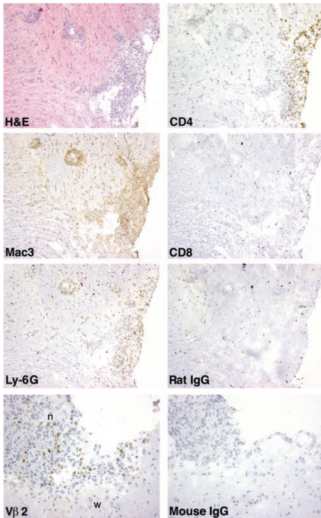
Figure 6. Immunohistochemical analysis of inflammatory infiltrates in brainstem and cranial nerve root. Frozen sections of brainstem from an irradiated Tg mouse with EAE (grade 2) induced by MS2-3C8 (B6) Tg T cells were stained for hematoxylin and eosin, CD4, Mac3, CD8, Ly-6G, and isotype control mAbs. Cranial nerve root (n) and brainstem (w) were stained with anti-V \beta 2 and isotype control mAbs.
