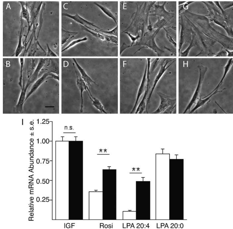
Figure 8. PPAR \gamma agonists elicit phenotypic modulation and dedifferentiation of VSMCs in vitro . VSMC cultures established in the presence of 2 ng/ml IGF-1 (A) were treated with 1 \mu\text{M} of each LPA 20:0 (C), LPA 20:4 (E), and Rosi (G) for 3 d. LPA 20:4 and Rosi treatments lead to a pronounced change in the morphology of VSMCs. Pretreatment of the cultures with 200 nM GW9662 for 30 min did not affect the spindle-like morphology of the IGF-1- (B) and LPA 20:0-treated cultures (D). In contrast, GW9662 reversed the flattened morphology into a spindle-like shape in cultures treated with LPA 20:4 (F) and Rosi (H, calibration bar 100 \mu\text{m} ). Expression of hCAD mRNA decreased significantly by day 5 in VSMCs treated with Rosi and LPA (I, white bars) compared with the IGF-treated control cultures. This trend was reversed in cultures pretreated with 200 nM GW9662 (I, black bars) as the PPAR \gamma antagonist caused a significant increase in the abundance of hCAD mRNA measured by quantitative RT-PCR ( P < 0.01 , ANOVA).
