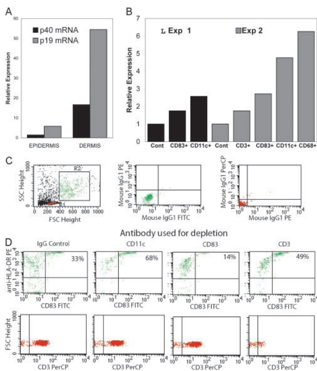
Figure 3. p19 and p40 gene expression in disperse split skin and dermally derived inflammatory cells. (A) Dermis from psoriasis lesions has greater p19 and p40 mRNA than epidermis. The data are from one representative experiment. A repeat run produced almost identical results. RNA was isolated from disperse split lesional skin taken from psoriatic plaques from two patients. RT-PCR for the p19 and p40 genes was performed on the epidermis and dermis and gene expression levels are shown relative to the hARP gene. In two other patients, the dermis was cultured for an addi-
