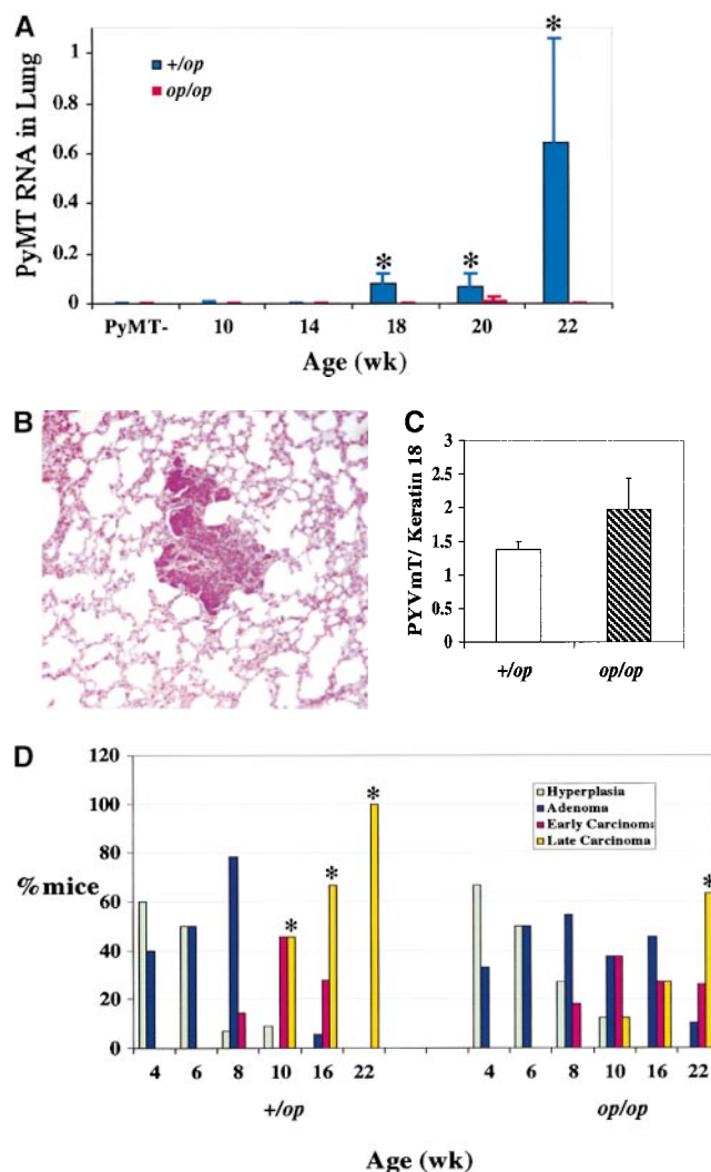
Figure 2. Histopathological progression and metastasis of mammary tumors in Csf1^{op}/Csf1^{op} PyMT mice was delayed. (A) Pulmonary metastasis of mammary tumors in + / Csf1^{op} and Csf1^{op}/Csf1^{op} PyMT mice was compared by Northern analysis of PyMT mRNA expression in lungs. Data are presented as the mean \pm SE of at least three mice for each time point. Asterisks indicate the significant difference of + / Csf1^{op} PyMT mice between 10 to 14 and 18 to 22 wk of age (Mann-Whitney test, P = 0.0016 , n = 21 ), and the significant difference between + / Csf1^{op} and Csf1^{op}/Csf1^{op} PyMT mice from 18 to 22 wk of age (Mann-Whitney test, P < 0.0001 , n = 28 ). (B) Hematoxylin and eosin–stained lung section from a + / Csf1^{op} PyMT mouse at 18 wk of age (original magnification: \times 100 ). (C) PyMT mRNA levels in mammary gland epithelium of + / Csf1^{op} and Csf1^{op}/Csf1^{op} PyMT mice from 6 to 12 wk of age were compared using Northern analysis. Mean \pm SE of eight mice/group. No significant difference was found between the two groups (unpaired Student's t test). (D) Histopathological progression of primary tumors to late carcinoma in Csf1^{op}/Csf1^{op} PyMT mice was delayed compared with + / Csf1^{op} littermates. Data are presented as the percentile distribution of primary tumors of + / Csf1^{op} ( n = 68 ) and Csf1^{op}/Csf1^{op} PyMT mice ( n = 70 ) in four histopathological stages at the ages indicated. Asterisks indicate a significant difference in the frequency of late carcinoma stage tumors in mice older than 8 wk of age compared with mice of the same genotype at 8 wk of age (Fisher's exact test, P = 0.0087 , 0.0004 , and 0.0006 for + / Csf1^{op} and P = 0.42 , 0.077 , and 0.0006 for Csf1^{op}/Csf1^{op} PyMT mice at 10, 16, and 22 wk of age, respectively).
