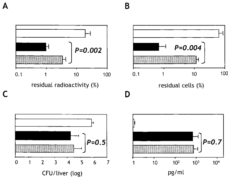
Figure 2. Vav1 is required for antitumor activity but not for antibacterial activity. (A) Mice (five wt , four Vav1 -/- , three Rag2/γC -/- ) were injected intravenously with 10^5 ^{51}\text{Cr} -labeled RMA-S cells. 4 h after injection, the residual radioactivity was measured in the lungs and is expressed as percentage of the total radioactivity. Data are representative of three separate experiments. (B) Mice (eight wt , five Vav1 -/- , six Rag2/γC -/- ) were injected intravenously with 2.5 \times 10^5 labeled RMA-S cells. 48 h after injection, cells in the peritoneal exudate were collected, enumerated, and stained with \alpha -CD3 and \alpha -H-2K k . Residual RMA-S cells were discriminated by virtue of size and surface phenotype (large CD3 + H-2K k cells). (C) Mice (six wt , six Vav1 -/- , four Rag2/γC -/- ) were injected intravenously with 10^4 L.m. , and 48 h later liver CFUs were enumerated. (D) The sera from mice infected with L.m. (10 wt , 11 Vav1 -/- , 4 Rag2/γC -/- ) were collected after mice were killed, and IFN- \gamma was detected by standard ELISA technique. P values (Student's t test) are expressed for Vav1 -/- versus wt . White bars, Rag2/γC -/- ; black bars, wt ; gray bars, Vav1 -/- .
