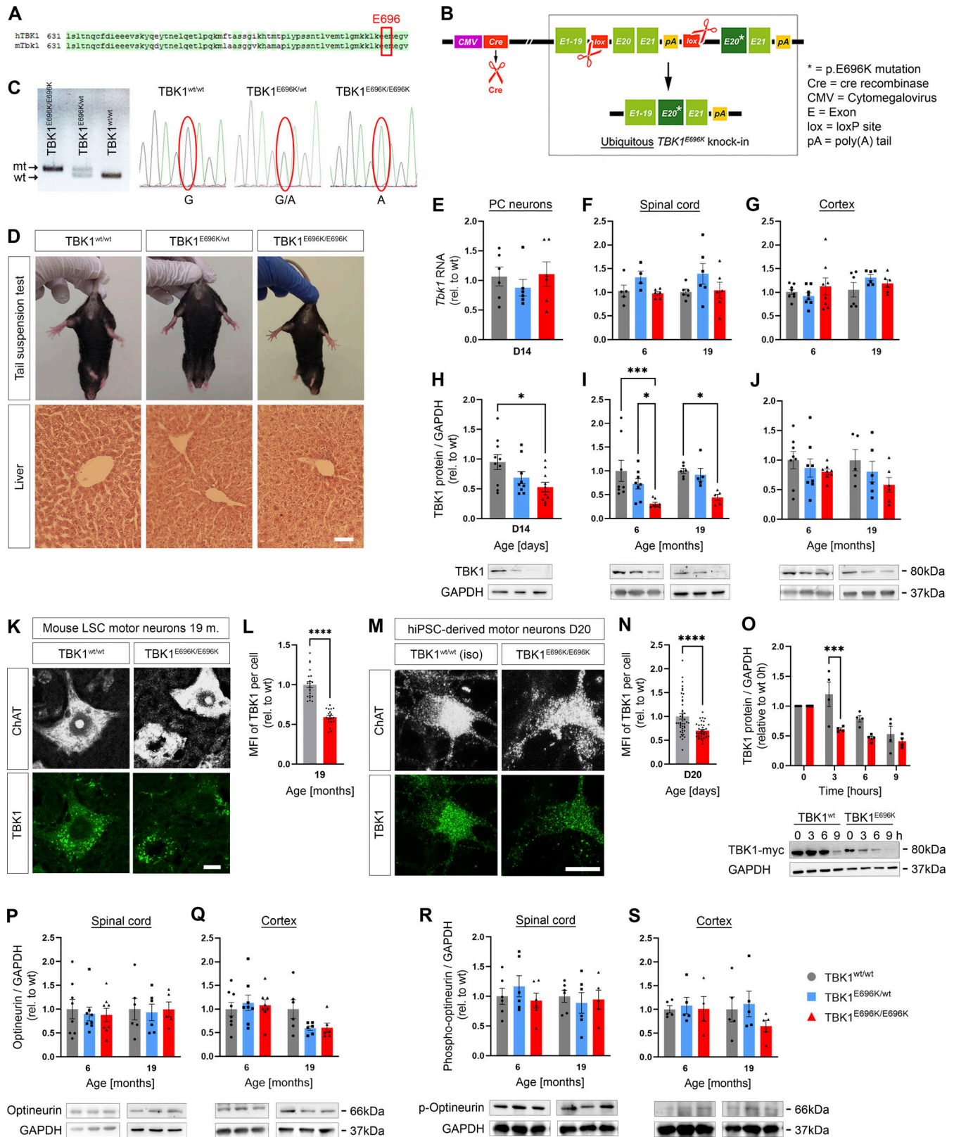
Figure 2. Generation and characterization of TBK1 E696K knock-in mice. (A) Conservation of p.E696 in TBK1 between mouse and human. (B) Scheme showing the generation of mice with constitutive global knock-in of the TBK1 E696K variant using the Cre/Lox system and a “mini-gene” approach. (C) PCR and sequencing of the wt and mutant bands of ear tissue from TBK1 E696K knock-in and wt siblings. (D) Representative photomicrographs of 19-mo-old male mice and light microscopic images of HE-stained livers show no morphological differences between the three genotypes. Scale bar: 100 \mu m. (E–G) Quantification of Tbk1 RNA expression by qPCR in mouse primary cortical (PC) neurons, spinal cord, and cortex tissue. Mean \pm SEM of n = 6 embryos of mixed sex per genotype from more than three independent experiments; one-way ANOVA with Tukey’s post hoc test in E. Mean \pm SEM of n = 4 –8 male mice per genotype; two-way
