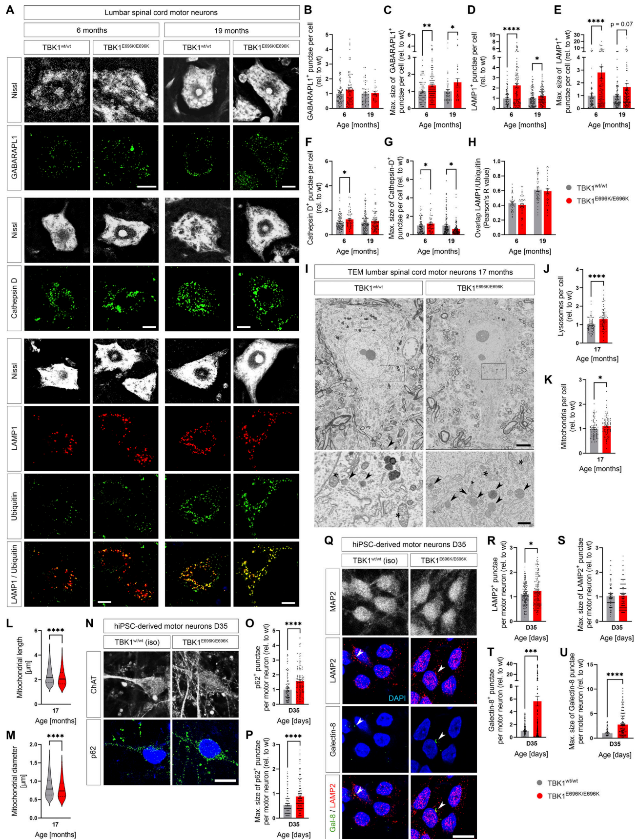
Figure 5. TBK1 E696K/E696K knock-in causes (presymptomatic) lysosomal pathology in mice and hiPSC-derived human motor neurons. (A) Representative photomicrographs of lumbar anterior horn motor sections from 6- and 19-mo-old homozygous TBK1 E696K knock-in and wt mice stained against
