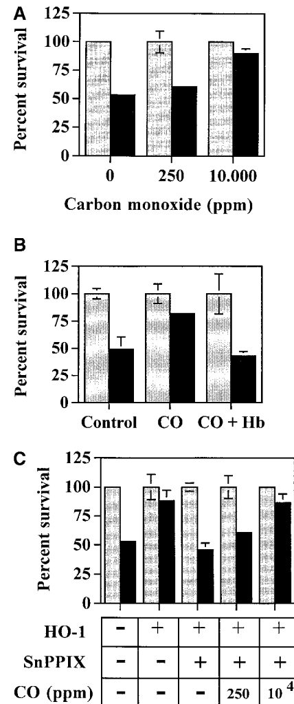
Figure 5. Exogenous CO suppresses EC apoptosis in the absence of HO-1. (A) 2F-2B ECs were transfected with a \beta -galactosidase expression vector and exposed to exogenous CO. Gray bars represent ECs treated with Act.D alone and black bars represent ECs treated with TNF- \alpha plus Act.D. (B) 2F-2B ECs were transfected with a \beta -galactosidase expression vector and exposed to exogenous CO (10,000 ppm) with or without Hb. Gray bars represent ECs treated with Act.D and black bars represent ECs treated with TNF- \alpha plus Act.D. (C) 2F-2B ECs were cotransfected with \beta -galactosidase and HO-1 ( \beta -actin/HO-1) expression vectors. Where indicated (+), HO-1 enzymatic activity was inhibited by SnPPIX and/or exposed to exogenous CO. Gray bars represent ECs treated with Act.D and black bars represent ECs treated with TNF- \alpha plus Act.D. Results shown (A, B, and C) are the mean \pm SD from duplicate wells taken from one representative experiment out of three.
