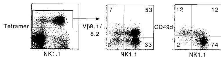
Figure 6. A subset of CD1d1-αGalCer tetramer+ cells are NK1.1- and express upregulated levels of CD49d. Liver lymphocytes from normal C57BL/6 mice were stained with tetramer-Cychrome, NK1.1-PE, and anti-Vβ-FITC or CD49d-FITC. Note that most tetramer+ NK1.1+ cells were CD49d- whereas tetramer+ NK1.1- cells were CD49d+. Both subsets exhibited the same bias in Vβ8 (middle) and Vβ7 and Vβ2 (not shown). Similar results were found for splenocytes and in Vα14-Jα281 TCR α chain transgenic mice.
