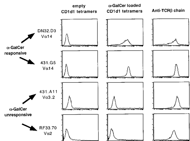
Figure 3. CD1d1- \alpha GalCer tetramers specifically stained V \alpha 14-J \alpha 281 NKT cell hybridomas. "Empty" or \alpha GalCer-loaded tetramers and anti-TCR- \beta mAb were used to stain two canonical V \alpha 14-expressing, \alpha GalCer-responsive hybridomas (DN32D3 and 431G5), one CD1d1-restricted \alpha GalCer-unresponsive V \alpha 3.2 hybridoma (431A11), and one K \beta -restricted V \alpha 2 hybridoma (RF33.70).
