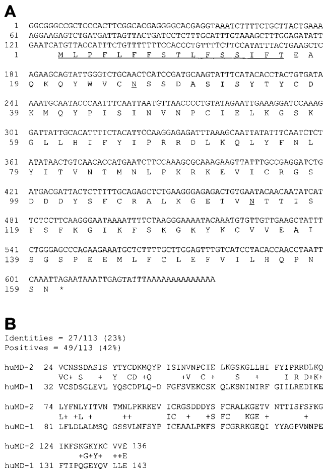
Figure 1. The nucleotide sequence of human MD-2 and its similarity to human MD-1. (A) The nucleotide sequence is shown with a deduced amino acid sequence. The signal peptide and canonical N -glycosylation sites are underlined. The stop codon is denoted by an asterisk. The nucleotide sequence of MD-2 will appear in the EMBL/GenBank/DBJ nucleotide sequence databases under accession no. AB018549. (B) Amino acid sequences of human MD-1 and MD-2 were aligned using the BLAST2 program at the National Center for Biological Information (Bethesda, MD).
