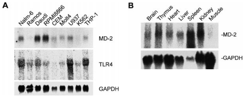
Figure 2. Expression of the MD-2 transcript. (A) Total RNA (20 \mu g/lane) from the indicated human cell lines was electrophoresed and hybridized with probes for human MD-2, TLR4, and GAPDH as indicated. Nalm-6, Ramos, Daudi, and RPMI8866 are of B lymphocyte lineage. CEM and Molt4 are of T cell origin. U937 and THP-1 are of monocytic origin. K562 is the erythroleukemia line. (B) Total RNA (20 \mu g/lane) from the indicated mouse tissues was used for Northern hybridization. The cDNA clone encoding mouse MD-2 was used as a probe. For GAPDH, the rat cDNA clone was used.
