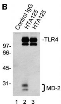
Figure 4. MD-2 is coprecipitated with TLR4. (A) Stable transfectants expressing MD-2 alone or with TLR4 were stained with or without cell permeabilization. The intracellular MD-2 precursor was stained with the anti-protein C mAb. The specificity of the anti-TLR4 mAb was shown by cell surface staining of stable transfectants. Goat anti-mouse IgG-FITC was used as the second reagent. Dotted lines correspond to histograms stained with the second reagent alone. Panels correspond to the original Ba/F3 line, a transfectant expressing TLR4 alone, and a transfectant expressing TLR4 + MD-2, respectively. (B) Stable transfectants expressing TLR4 and
