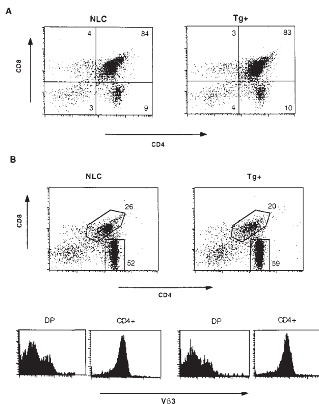
Figure 6. Normal positive selection in dnJNK1 transgenic mice. (A) Cell surface staining for CD4 and CD8 in total thymocytes from dnJNK1 transgenic (line 44) ( Tg + ) or negative littermate control ( NLC ) mice was analyzed by flow cytometry. The numbers represent the percentage of cells in each quadrant. (B) Total thymocytes from Cyt c TCR transgenic mice ( NLC ) or Cyt c TCR × dnJNK1 double transgenic mice ( Tg + ) were analyzed for CD4 and CD8 expression in the total thymus ( top ) and V \beta 3 expression in the DP or single CD4 + gates ( bottom ). The numbers indicate the percentage of DP CD4 + CD8 + and SP CD4 + cells in the total thymus.
