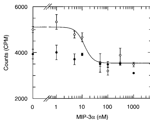
Figure 9. Competition binding of [ ^{125}\text{I} ] MIP-3 \alpha to HEK 293 cells transiently transfected with DCCR2. Binding assays were performed as described in Materials and Methods. Open circles denote binding to pcDNA3.1(+) DCCR2 transfectants; closed circles denote binding to pcDNA3.1(+) CAT transfectants.
