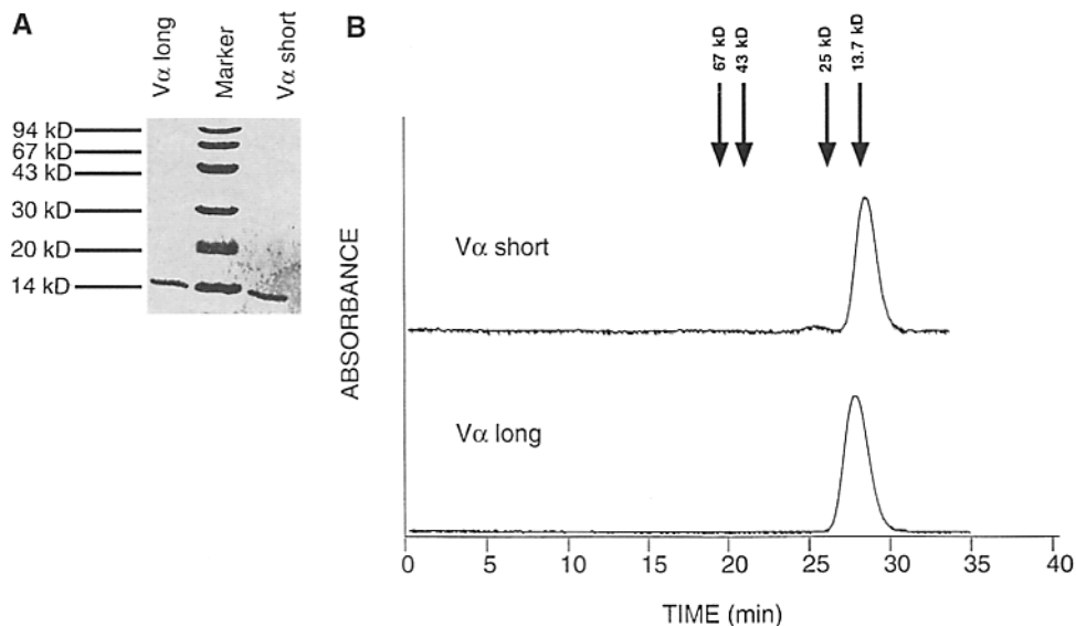
Figure 2. Homogeneity of refolded V\alpha domains. (A) SDS-PAGE of purified V\alpha 2 domains. Both V\alpha long and V\alpha short were expressed in E. coli as described in Materials and Methods, and protein was refolded and purified through both ion exchange and size exclusion chromatographic steps as described. The TCR domains were examined after reduction of disulfide bonds in 20% polyacrylamide gel containing SDS. The molecular size markers are indicated in kilodaltons. (B) Size exclusion chromatography under native conditions. Samples of the refolded V\alpha domains were analyzed by size exclusion chromatography in PBS on Superdex 75L at a flow rate of 0.5 ml/min. Positions of molecular size standards are indicated in kilodaltons. Absorbance at 280 nm is plotted in arbitrary units.
