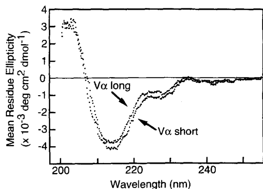
Figure 3. CD spectra of refolded V\alpha domains. CD spectra were collected as described in Materials and Methods at 25°C. Spectra of V\alpha long and V\alpha short are indicated.
