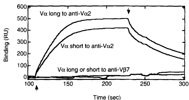
Figure 4. V\alpha 2 domains bind to anti- V\alpha 2 but not anti- V\beta 7 mAb. Anti- V\alpha 2 or anti- V\beta 7 mAb was coupled to a biosensor chip ( \sim 8,000 RU of each were coupled) as described in Materials and Methods. V\alpha long or V\alpha short was injected over the two mAbs at a flow rate of 10 \mu l/min , and binding was detected by SPR. The upward-pointing arrow indicates the initiation of the wash-on (association) phase, and the downward arrow indicates the initiation of the wash-out (dissociation) phase.
