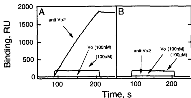
Figure 5. Failure to detect dimerization in SPR assay. (A) V \alpha short was immobilized on a biosensor surface (to level of \sim 3,000 RU) as described in Materials and Methods and exposed to either the V \alpha short domain in solution or an anti-V \alpha 2 mAb as indicated at a flow rate of 10 \mu\text{l}/\text{min} . B shows a blank surface. The concentration of anti-V \alpha 2 was 100 nM, and the concentration of the solution phase V \alpha short domain was injected at a concentration of either 100 nM or 100 \mu\text{M} .
