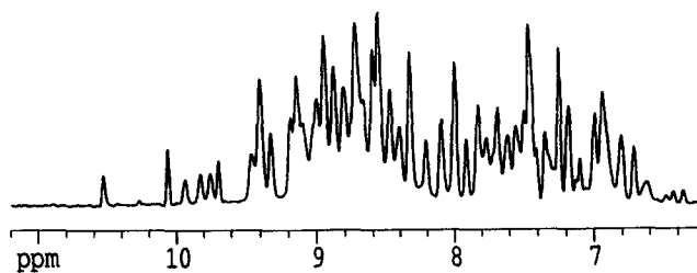
Figure 6. ^1\text{H} NMR spectrum of the amide region of V \alpha short, recorded from a 0.25\text{-mM} solution at 600 \text{ MHz} , 25^\circ\text{C} . The transverse relaxation rates for backbone amide protons were used to determine the rotational correlation time, \tau_c , of the protein, as described in Materials and Methods.
