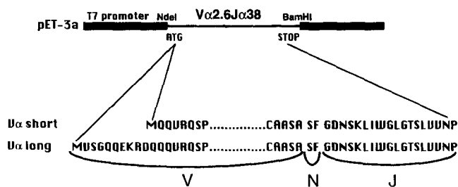
Figure 1. Structure of V \alpha long and V \alpha short expression vectors. A schematic of the pET3a subclones of V \alpha short and V \alpha long is shown. Partial amino acid sequences emphasizing the NH _2 termini, the N regions of the encoded proteins, and the J segments are shown.
