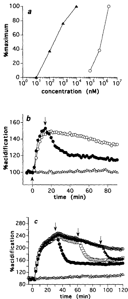
Figure 3. Short-lived peptide–MHC complexes produce a transient increase in T cell acidification. (a) The increase in acid release is proportional to the log of peptide concentration (see also Fig. 1 b ). Shown are acidification dose responses for B10A.F2 T cells exposed to (○) MBP Ac(1-14) and (▲) Ac(1-14)4A normalized to the % acidification after 30 min exposure to the at maximum peptide concentration. Half-maximal proliferation for MBP Ac(1-14) and Ac(1-14)4A is obtained at peptide concentrations of 10 μM and 1 nM, respectively. (b) The acidification rates of a mixture of B10A.F2 T cells and APCs briefly exposed to (○) 10 μM MBP Ac(1-14)4A, (●) 100 μM MBP Ac(1-14), and (△) media. Peptide was added at t = 0 min (first arrow); at t = 15 min (second arrow) peptide addition was stopped and the chamber was continuously perfused with media. (c) The long-lived T cell response to MBP Ac(1-14)4A is sustained by active TCR ligation. Mixtures of B10A.F2 T cells and APCs were exposed to (●, □, ▲) 1 μM MBP Ac(1-14)4A or (△) media for 30 min. 10 μg/mL of the I-A k -specific 10-2.16 antibody was added (●) immediately, (□) 30 min, and (▲) 60 min after peptide exposure (first, second, and third arrows, respectively). Identical results were also obtained with 1 and 100 μg/mL 10-2.16 antibody (data not shown). L cells transfected with I-A k were used as APCs.
