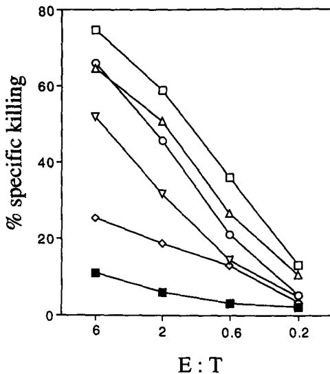
Figure 1. CTL can kill with comparable efficiency target cells in the presence of a very large range of peptide concentrations. Specific lysis of JY cells by clone CER43 in the absence (■) or in the presence of different concentrations of M58-66: 10 -7 M (□); 10 -9 M (Δ); 10 -11 M (○); 10 -13 M (∇); 10 -15 M (◇)
