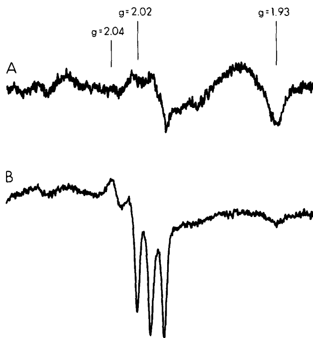
Figure 1. EPR spectra of spinal cords from naive mice at 20 K: (A) before exposure to NO, (B) after exposure to NO dissolved in acetonitrile (positive control). Experimental settings: microwave frequency, 9.4437 GHz; modulation frequency, 100 KHz; modulation amplitude, 6.3 G; microwave power, 0.64 mW.
