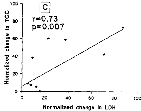
Figure 3. Scatterplot relating changes in LDH and TCC. Data pooled from the four experiments in which LDH and TCC were both measured, normalized by expressing maximum change from baseline in each experiment as 100% and all other results as percentage of this. Data shown for one normal serum (A; no significant correlation) and two NeF sera (B and C; Pearson's r as indicated). Other control sera also showed no significant correlation.
