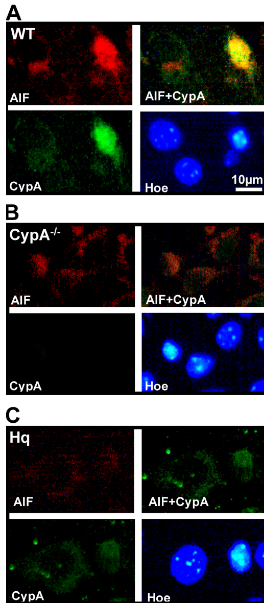
Figure 3. Nuclear translocation of AIF was impaired in the absence of CypA and vice versa. (A) Immunofluorescent labeling of AIF (red), CypA (green), and chromatin (HOECHST 33342; blue) 3 h after HI in WT type mice showing both strong AIF and CypA nuclear staining in an injured neuron, as judged by the condensed nuclear morphology. (B) Labeling, as in A, in CypA -/- mice showing very weak nuclear AIF staining in injured neurons. (C) Labeling, as in A, in AIF-deficient Hq mice showing very weak CypA staining in injured neurons compared with WT type mice. Bar, 10 μm.
