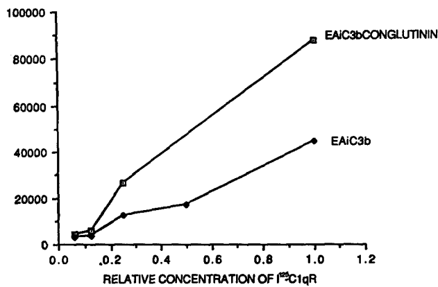
Figure 5. Binding of ^{125}\text{I} -labeled C1qR to EAiC3b cells in the presence or absence of conglutinin. EAiC3b cells were preincubated with (□) or without (◆) conglutinin as described in Materials and Methods, then exposed to ^{125}\text{I} -labeled C1qR in sodium barbital buffer (pH 7.4) containing 5% (wt/vol) glucose. Unbound ligand was separated and cpm bound to cells were measured on an LKB gamma counter.
