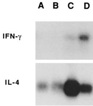
FIGURE 6. Effect of anti-IL-4 treatment on cytokine mRNA production during leishmaniasis. Poly(A) + RNA (10 μg) was isolated from the spleens of untreated or anti-IL-4-treated BALB/c mice (lanes A and B, respectively) or the popliteal lymph nodes of untreated or anti-IL-4-treated BALB/c mice (lanes C and D, respectively) 6 wk after infection with L. major . Northern hybridizations were performed using IL-4- and IFN-γ-specific probes.
