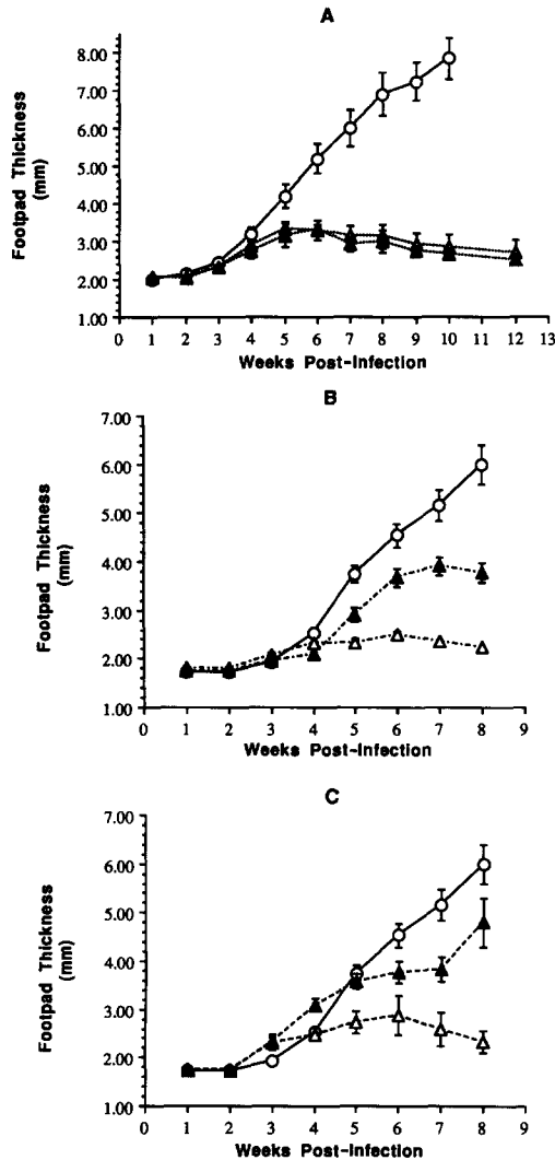
FIGURE 7. Effect of anti-IFN-γ on the progression of L. major infection. (A) Untreated BALB/c mice (○); anti-IL-4-treated (△); and anti-IL-4 + anti-IFN-γ-treated (▲) BALB/c mice. Footpad measurements represent the mean ± SEM from five mice. (B) Untreated BALB/c mice (○); C57BL/6 untreated (△); and anti-IFN-γ-treated (▲) mice. Footpad measurements represent the mean ± SEM from four mice. (C) Untreated BALB/c mice (○); GK1.5-BALB/c untreated (△); and anti-IFN-γ-treated (▲) mice. Footpad measurements represent the mean ± SEM from four mice.
