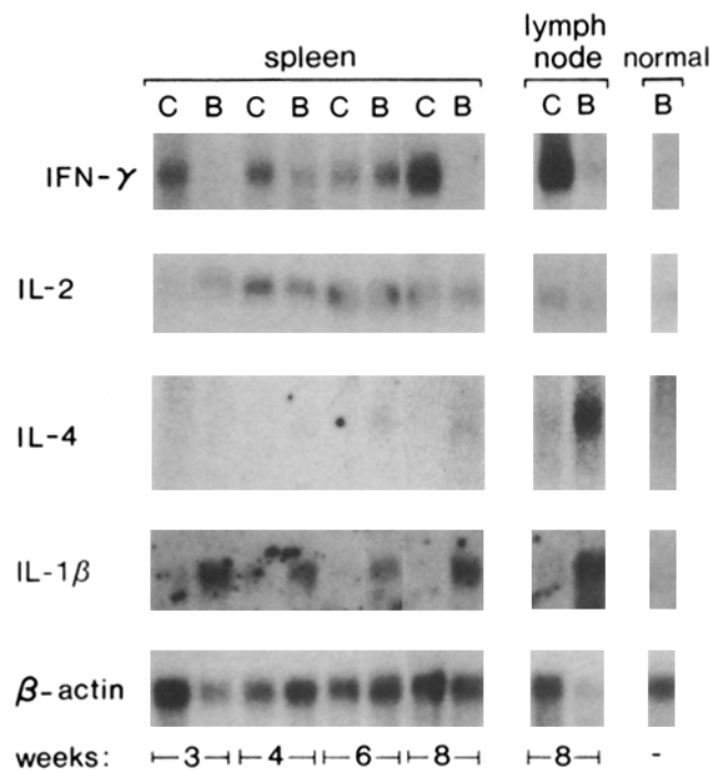
FIGURE 1. Cytokine mRNA during leishmaniasis. Poly(A) + RNA (5 µg) was isolated from the spleens and lymph nodes of BALB/c (B) and C57BL/6 (C) mice at designated times after infection with L. major . Northern hybridizations were performed using the indicated cytokine-specific probes (see Materials and Methods). Control RNA is from uninfected BALB/c spleen.
