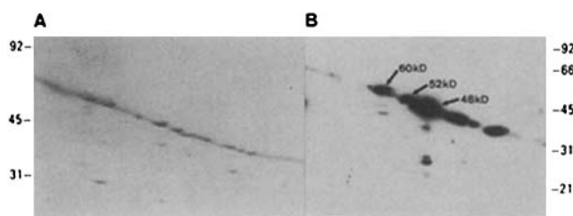
FIGURE 2. Partial proteolysis of HeLa cell extract by S.a. V8 protease. (A) Coomassie blue staining of two dimensional 15% polyacrylamide gel of cell extract digested with 10 µg/ml protease. (B) Immunoreactive fragments of the different proteins 60 kD, 52 kD, and SS-B (48 kD), as detected by antibody and ^{125}\text{I} -
