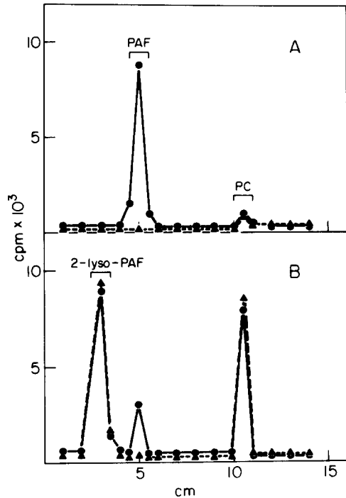
FIGURE 2. Representative TLC analysis of PAF synthesized by rat peritoneal macrophages stimulated for 1 h with 20 ng/ml of mTNF after 2 h preincubation with 15 \mu Ci/ml of [ ^3 H]acetyl-CoA (A) or with 0.1 mM unlabelled acetyl-CoA and 2 \mu Ci/ml [ ^3 H]2-lyso-PAF (B). The lipids were extracted from cells and supernatant (35) and analyzed by TLC using as solvent chloroform/methanol/acetic acid/water (50:25:8:4). The plates were divided into 30 sections of 0.5 cm each and counted as described in Materials and Methods. The pattern obtained with TNF-stimulated cells ( \bullet ) and control unstimulated cells ( \blacktriangle ) is shown. In parallel experiments, labeled PAF, PC, and 2-lyso-PAF were chromatographed as standards; the position of these compounds is indicated. Three experiments were performed with similar results on cell-associated and supernatant lipids.
