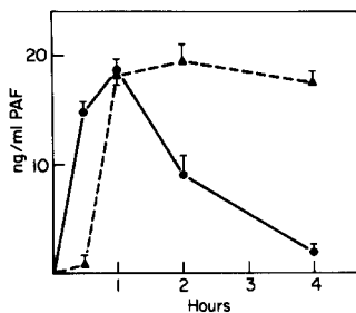
FIGURE 3. Time course of PAF synthesis and release by rat peritoneal macrophages stimulated with 20 ng/ml of mTNF. Cell-associated PAF ( \bullet ) and PAF released in the supernatant ( \blacktriangle ) are shown; 10^6 cells were used for each time point.
