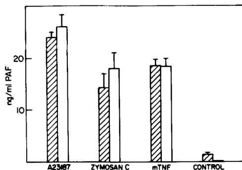
FIGURE 1. Synthesis and release of PAF by rat peritoneal macrophages treated for 1 h with 1 \mu g/ml of A23187, 0.2 mg/ml of zymosan C, 20 ng/ml of mTNF or untreated. 10^6 cells were used for each experiment. Cell-associated PAF, shaded columns; supernatant PAF, blank columns. In this and the following figures, PAF concentration is referred to 1 ml of cell culture medium and to the corresponding cell aliquot to allow comparison of the amount of PAF released with that remaining cell associated. Vertical bars indicate the standard deviation of the mean of different experiments ( n = 3 ). The assay of PAF was carried out in duplicate for each experiment.
