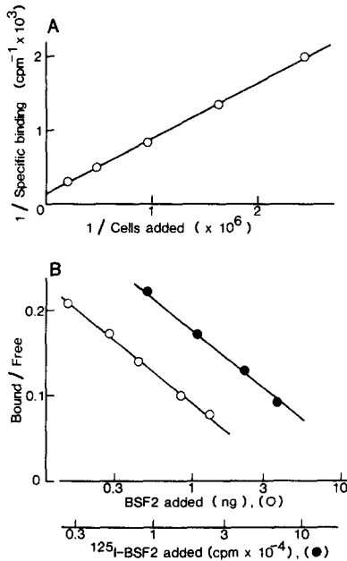
FIGURE 3. Determination of the maximal binding capacity and specific radioactivity of ^{125}\text{I} -BSF-2. (A) 9,300\ \text{cpm} of ^{125}\text{I} -BSF-2 was incubated for 150 min with five different concentrations of CESS cells (up to 5 \times 10^6 ) in the presence or absence of 200-fold excess amount of unlabeled BSF-2. Data (averages of duplicates) are plotted as reciprocal specific binding versus reciprocal cells added. The ordinate intercept of the regression line means the reciprocal counts that would bind at infinite number of cells (maximal binding capacity). (B) Self-displacement analysis is performed as described in Materials and Methods. 9,300\ \text{cpm} of ^{125}\text{I} -BSF-2 and increasing amounts of unlabeled BSF-2 (up to 1.3\ \text{ng} ) or ^{125}\text{I} -BSF-2 (up to 80,000\ \text{cpm} ) were incubated with 10^6 CESS cells. The mean specific binding of duplicates is plotted as a bound/free ratio (corrected for maximal binding capacity). The specific radioactivity is determined as mentioned in the text.
